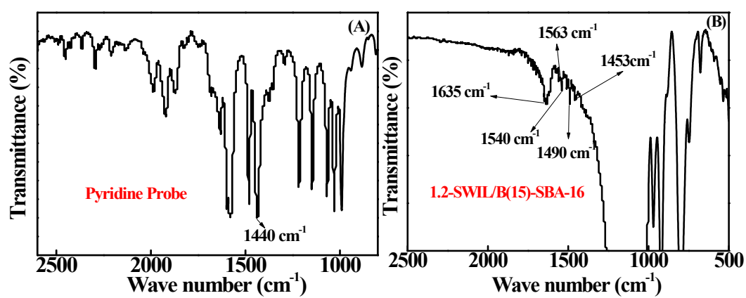
Fig. S2. The Py-IR spectra of samples using pyridine as probe (A) Pyridine and (B) 1.2-SWIL/B(15)-SBA-16.
