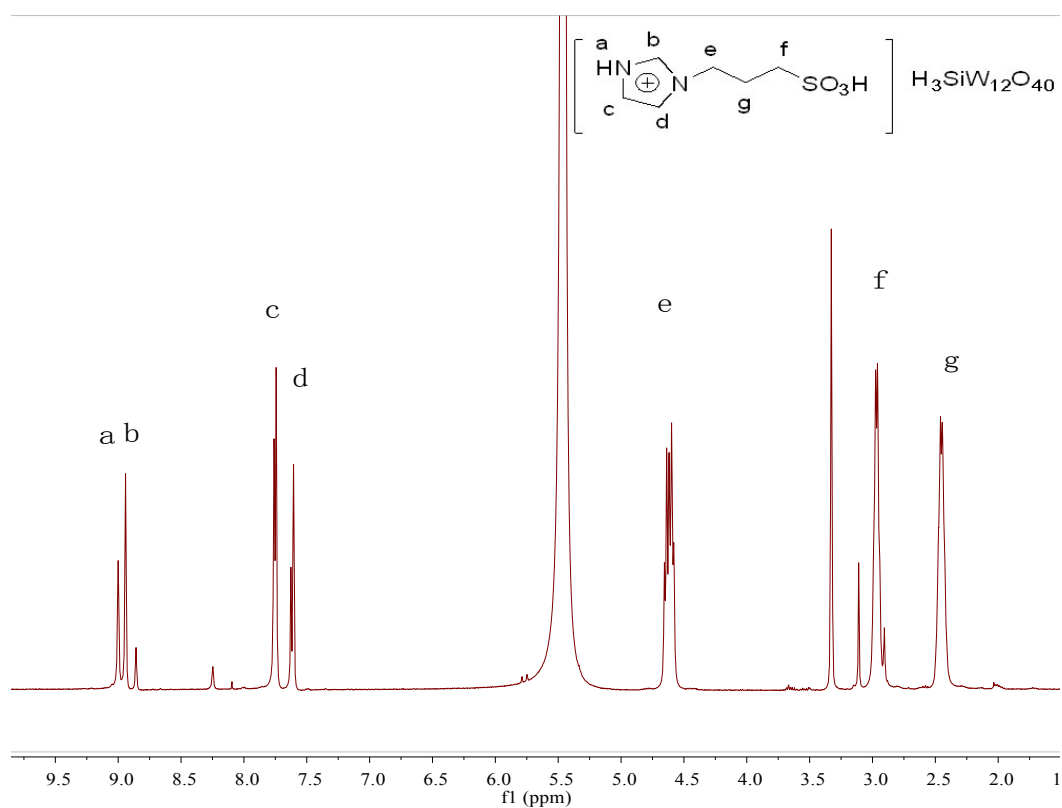
Fig. S1 The ^1\text{H} NMR spectrum of SWIL
