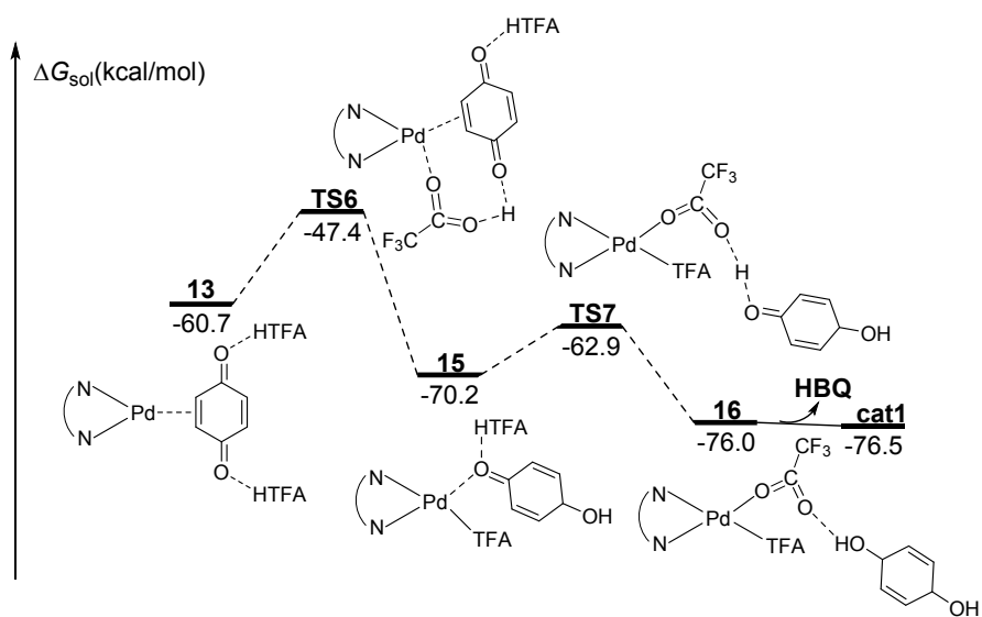
Fig. S1 Free energy profiles for the oxidation of Pd(0) to Pd(II) by BQ.
