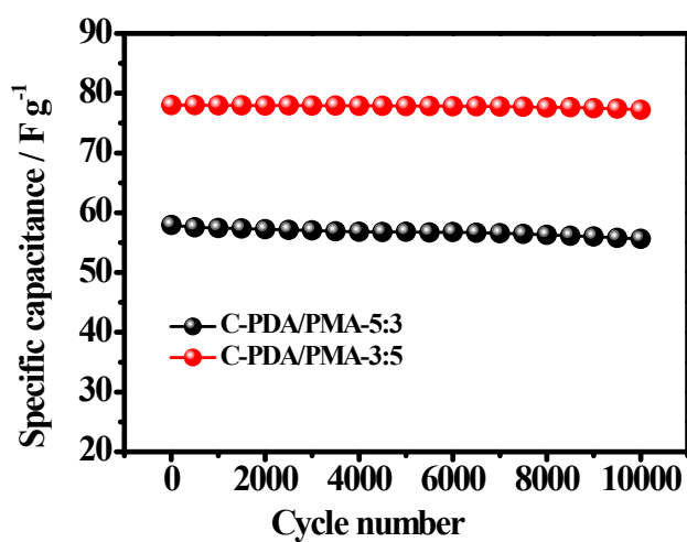
Figure S2. Electrochemical performance of the C-PDA/PMA-5:3, C-PDA/PMA-3:5 samples when tested in a two-electrode configuration.
