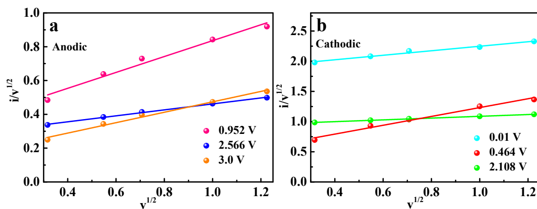
Figure S2 Fitting curves of i/v^{1/2} responses plotted against v^{1/2} for anodic scans (a) and cathodic scans (b).
