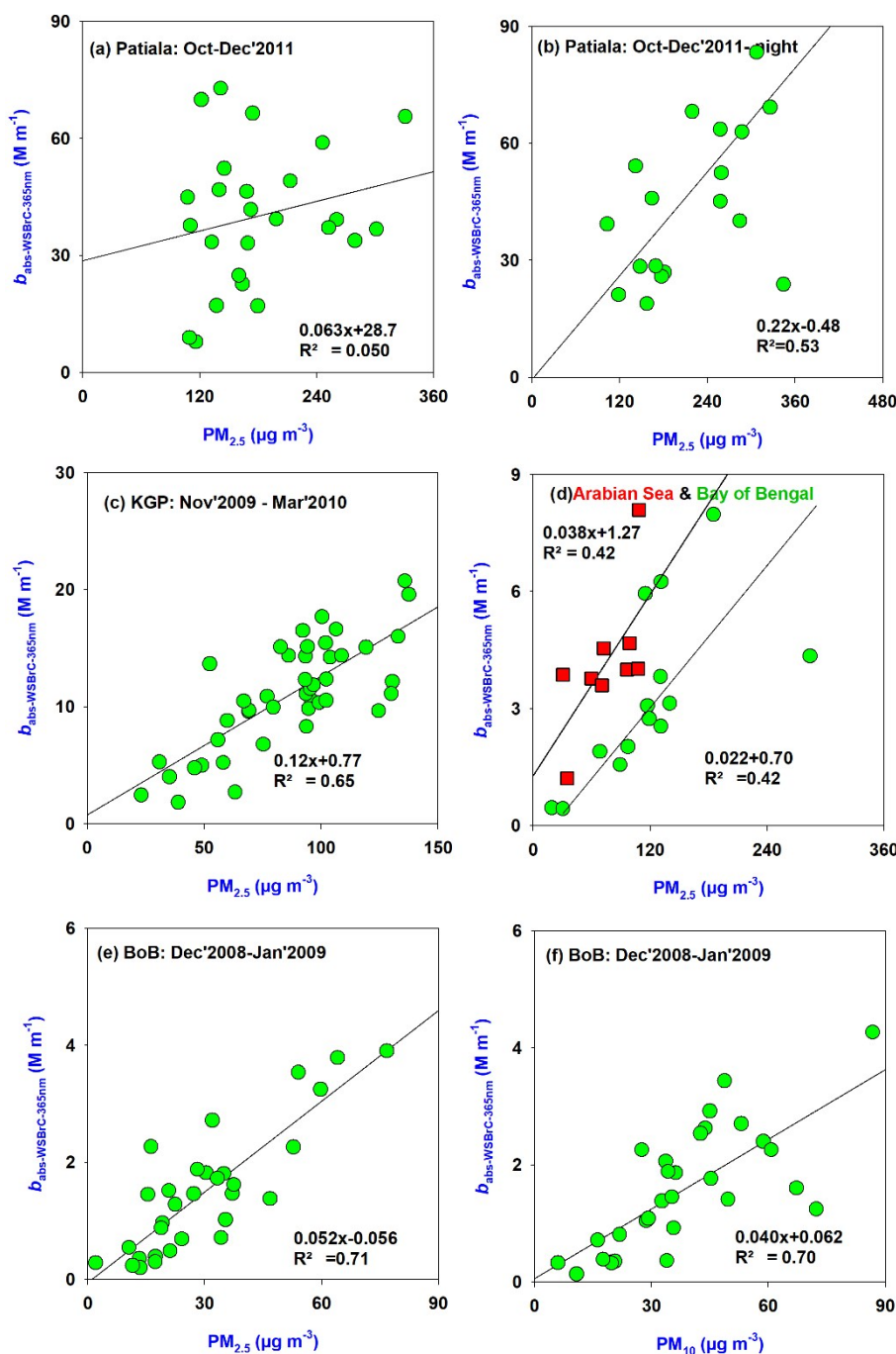
Figure S1: Linear relationships between mass absorption coefficient of water-soluble BrC at 365nm and particulate aerosol mass concentration in the Indo-Gangetic Plain outflow.
