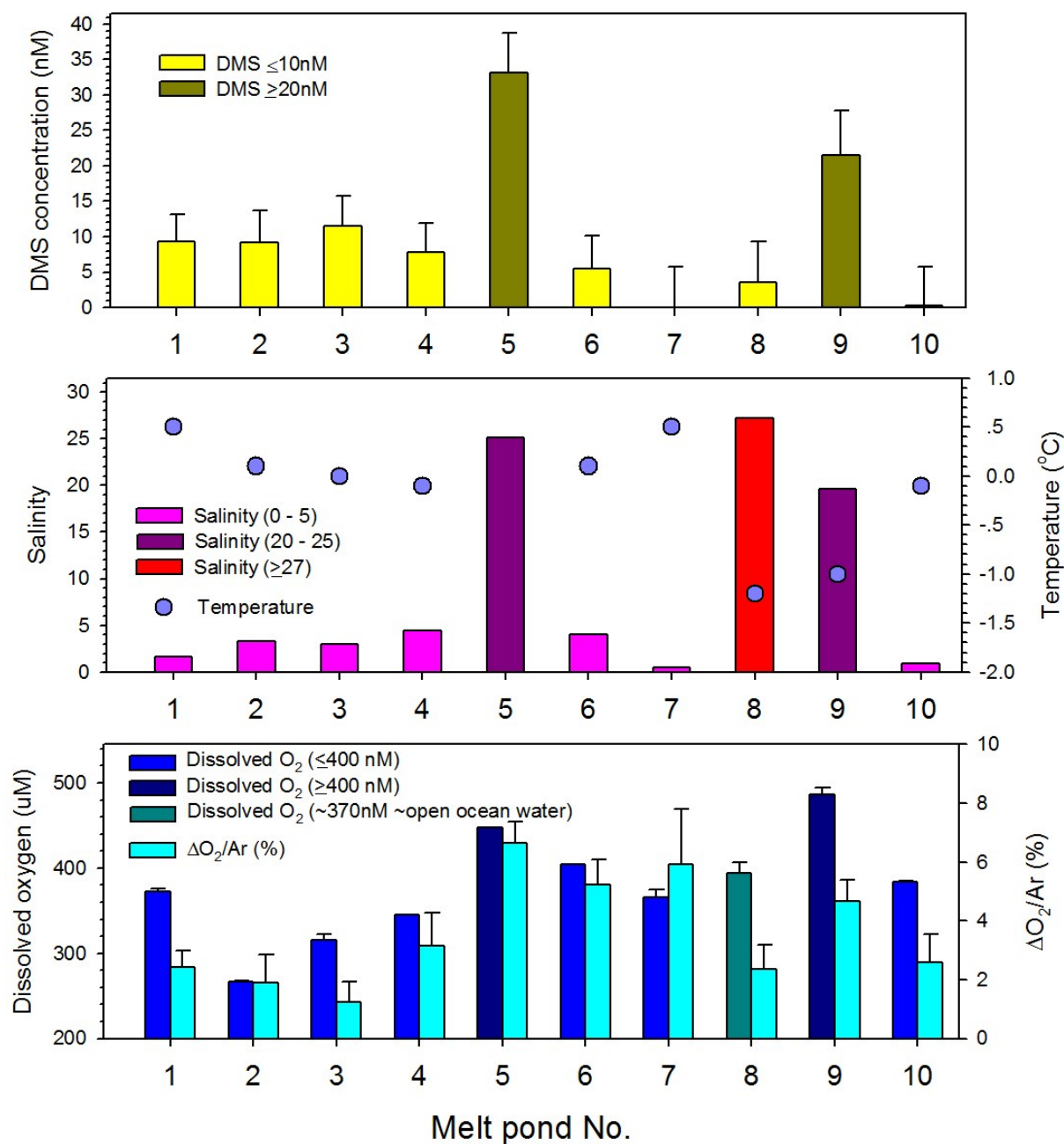
Supplementary Figure 1. Chemical and physical properties of each melt pond (*which is visualizing the data of Table 1)
