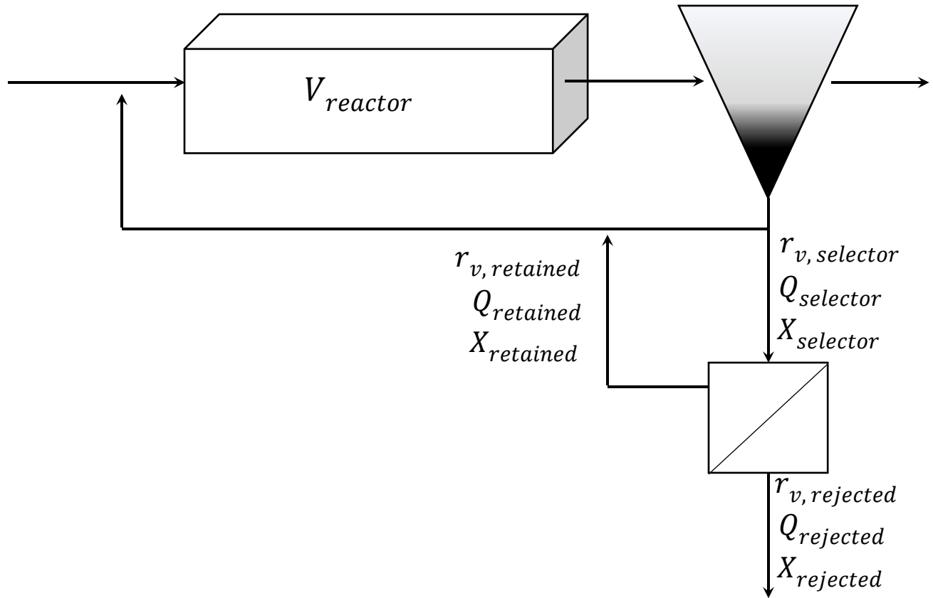
Figure A1. Basic schematic of a wastewater treatment plant with external selector.
