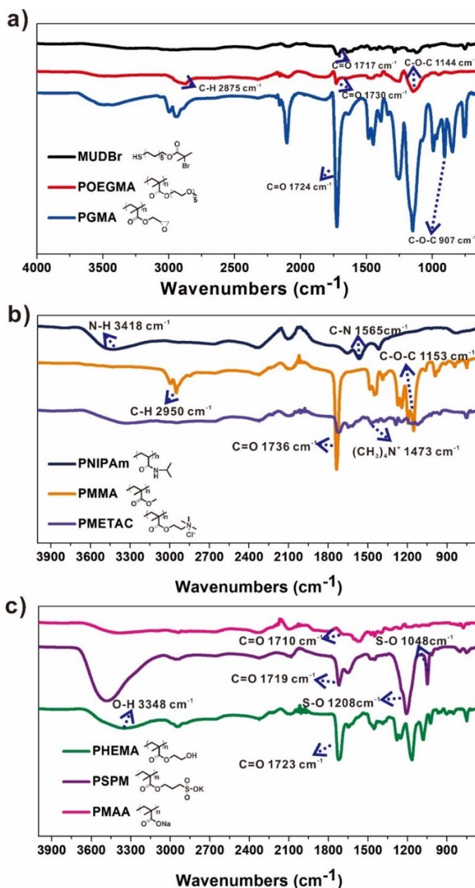
Fig. S1. (a-c) ATR-FTIR spectra of MUDBr SAM and various polymer brushes coated-Au substrates.
