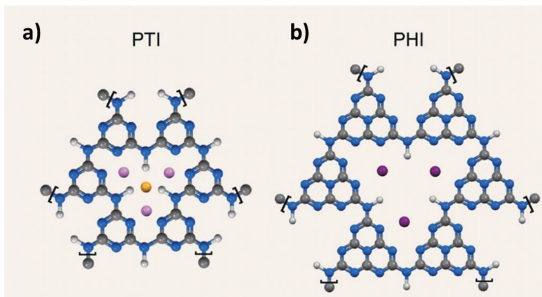
Figure S1. Idealized structure of a) PTI and b) PHI reproduced from ref. 3. Grey (C), blue (N), white (H), pink (Li), yellow (Cl) and purple (Na).
