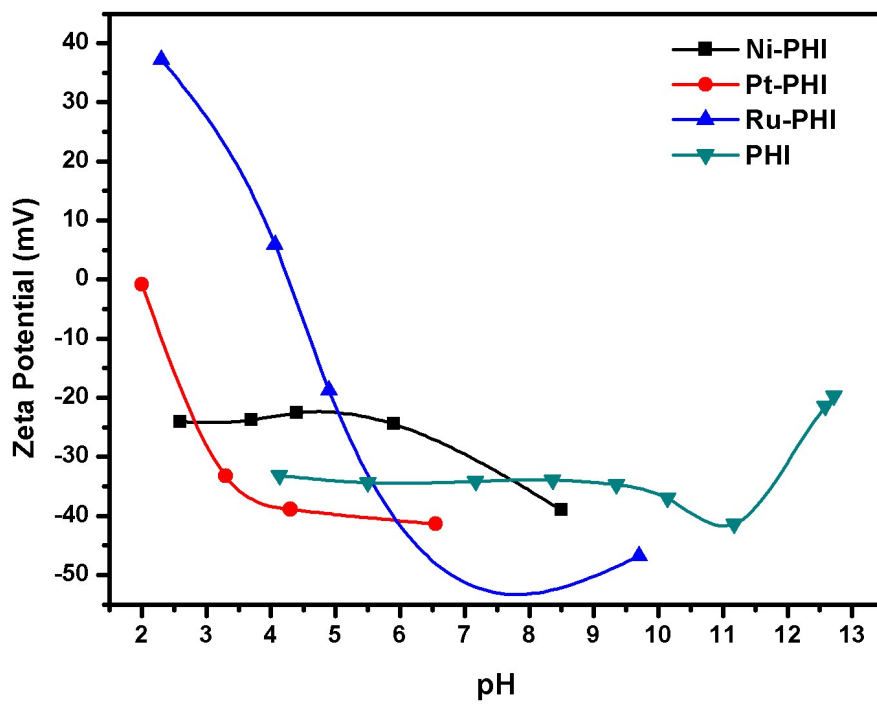
Figure S2. Zeta potential for the samples PHI, Pt-PHI, Ru-PHI and Ni-PHI.
