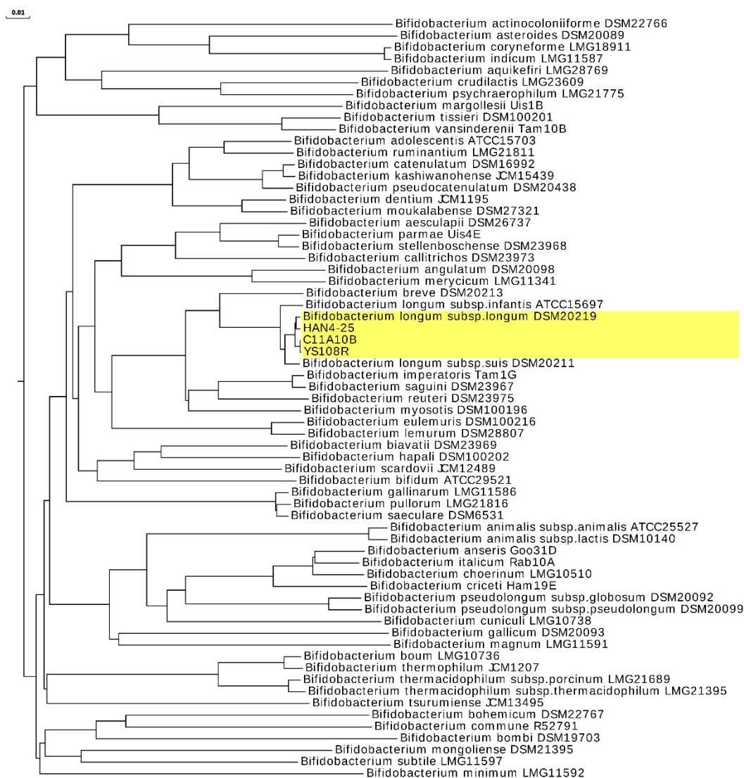
Fig. S1 Phylogenetic analysis based on genomic sequences
