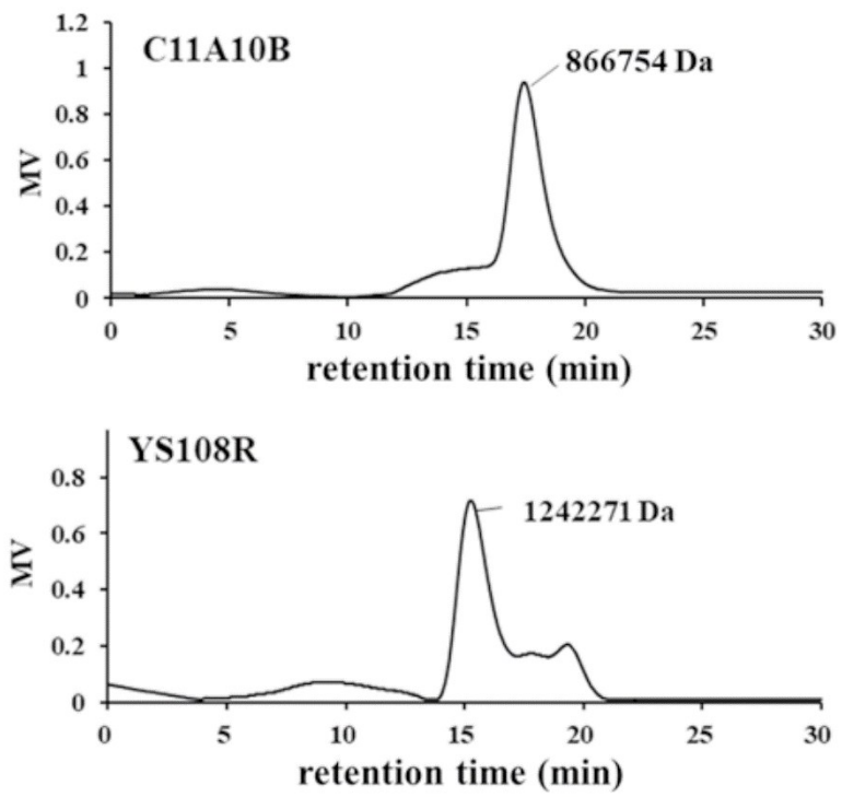
Fig. S2 Size exclusion chromatography analysis of EPS produced by B. longum C11A10B and YS108R
