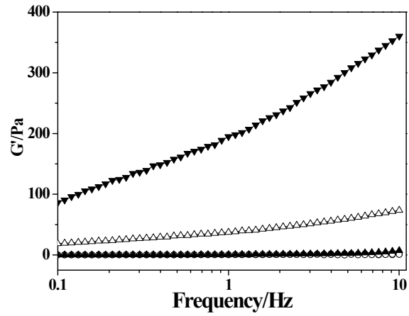
Figure S2. Frequency dependence of the storage modulus ( G' ) of mixed protein suspensions (10%, w/v) with different SP:CP ratios: 5:0 (●), 3:1 (○), 1:1 (▲), 1:3 (△), and 0:5 (▼).
