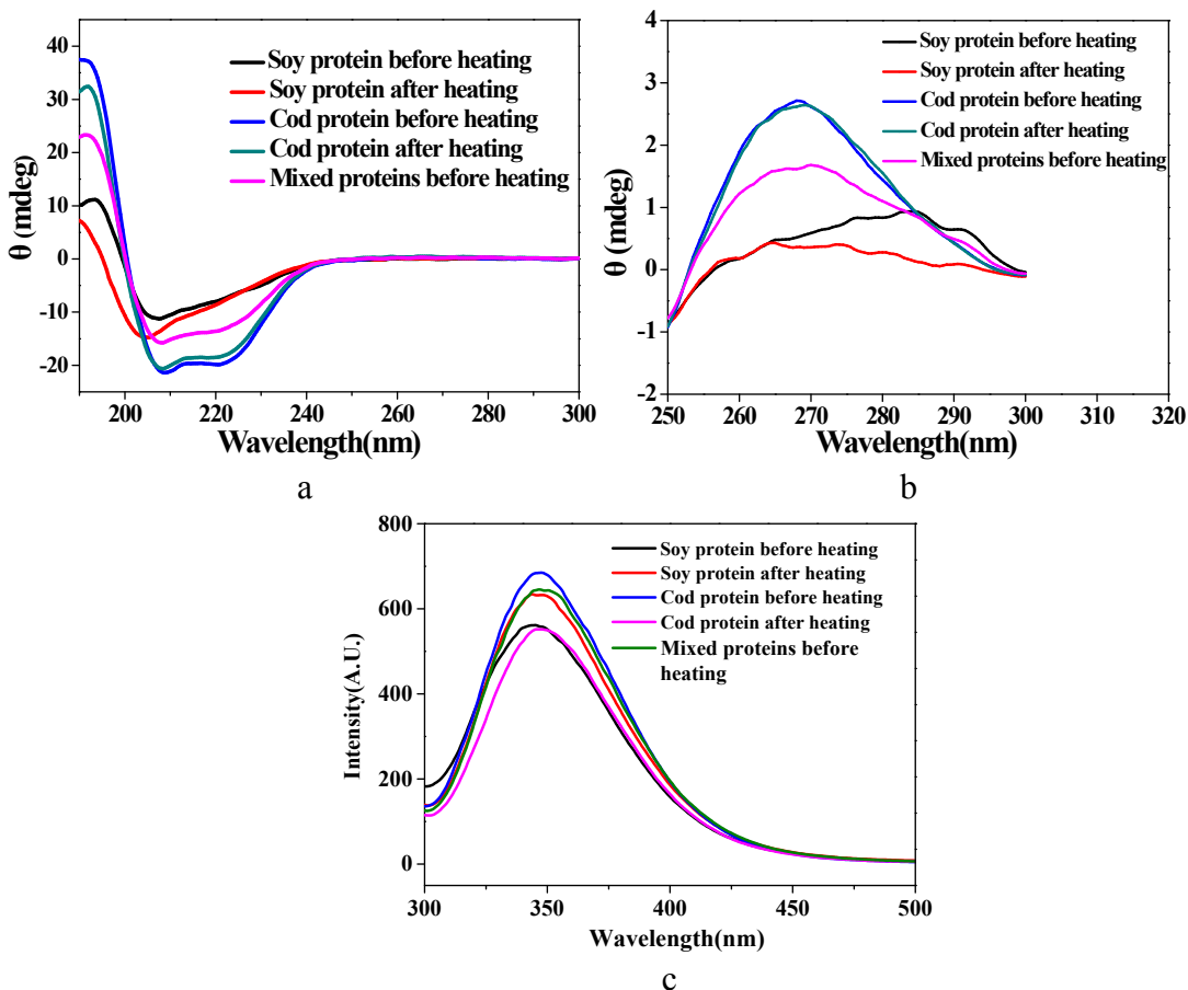
Figure S1. Spectroscopic characterization of soy protein and cod protein before and after heating, and the mixed proteins (1:1) before heating: a, far-UV CD, b, near-UV CD, c, fluorescence spectra.
