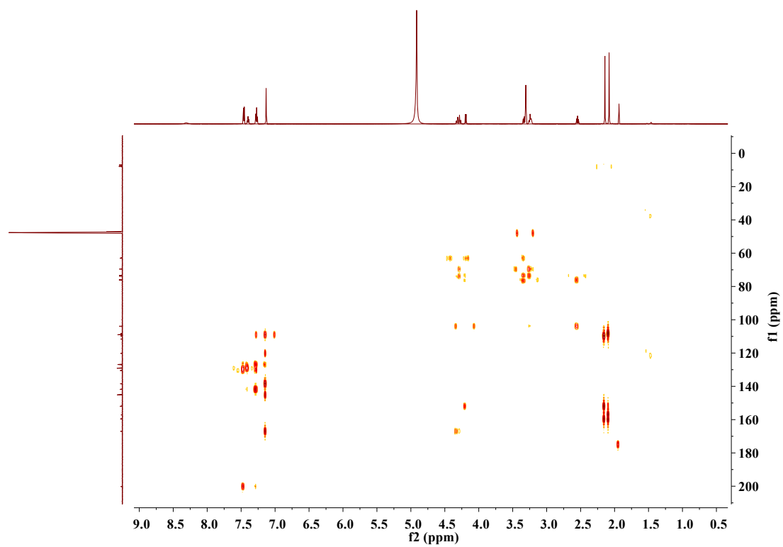
Fig. S1. The spectrum of HMBC.
