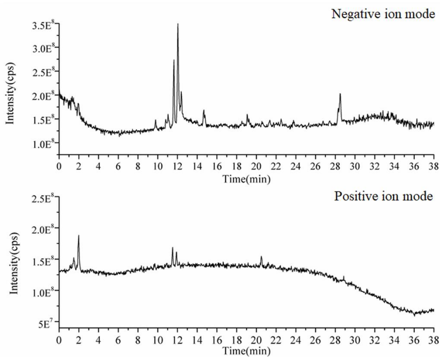
HPLC-ESI-MS total ion chromatogram of MWE analysed with negative and positive ion mode.
