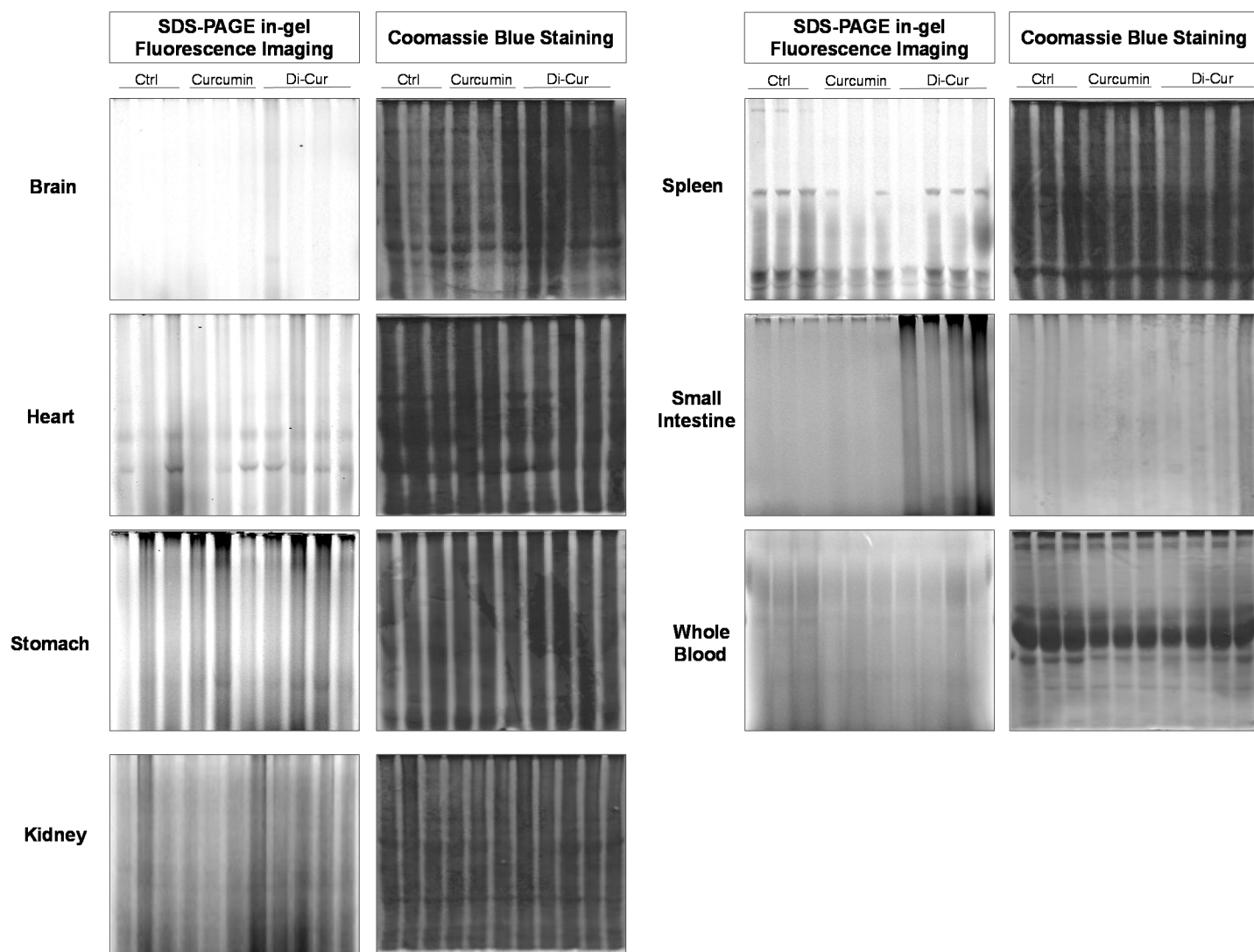
Figure S1. Effects of curcumin click-chemistry probe Di-Cur on labelling cellular proteins in tissues. Left panel: SDS-PAGE in-gel fluorescence. Right panel: Coomassie blue staining.
