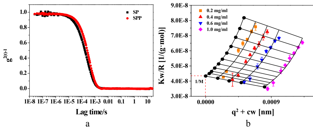
Figure S1. a, autocorrelation function obtained for dispersions of SP and SPP at the scattering angle 90^\circ . b, zimm plots of SPP in 10 mM pH 7.0 PBS at 25^\circ\text{C} .
