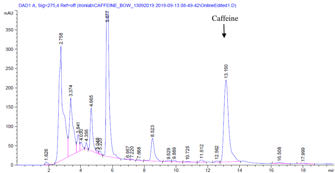
Fig. S3 HPLC profile of caffeine in the GTE-CUR drink.
