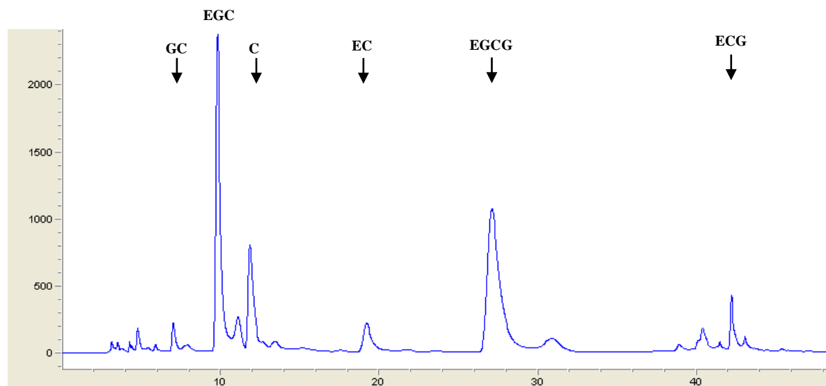
Fig. S1 HPLC profile of catechins in the GTE-CUR drink.
