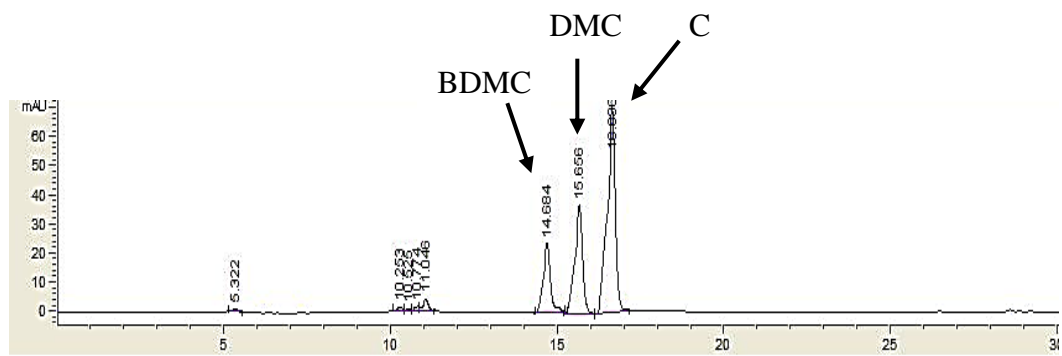
Fig. S2 HPLC profile of curcuminoids in the GTE-CUR drink.
