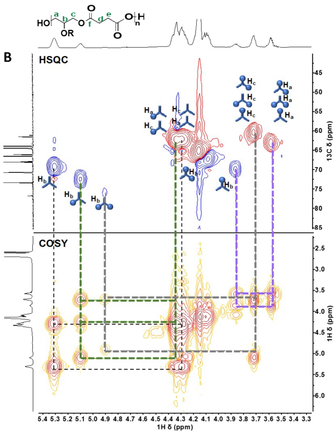
Figure S2 – Sections of the HSQC and COSY NMR spectra showing the assignments of glycerol units in a A) linear polymer synthesised in \text{scCO}_2 (entry 5, Table 1) and B) branched poly(glycerol succinate) polymer synthesised in the melt (entry 8, Table 2). The combination red-blue for HSQC and yellow-red for COSY are reported simply to distinguish the two types of spectra. For glycerol branching representations refer to Scheme 2 .
