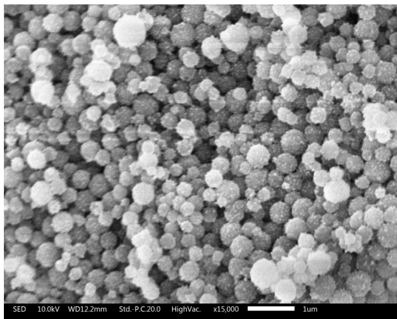
Figure S4 SEM images of LPR@Ag-10 nanocomposites.
