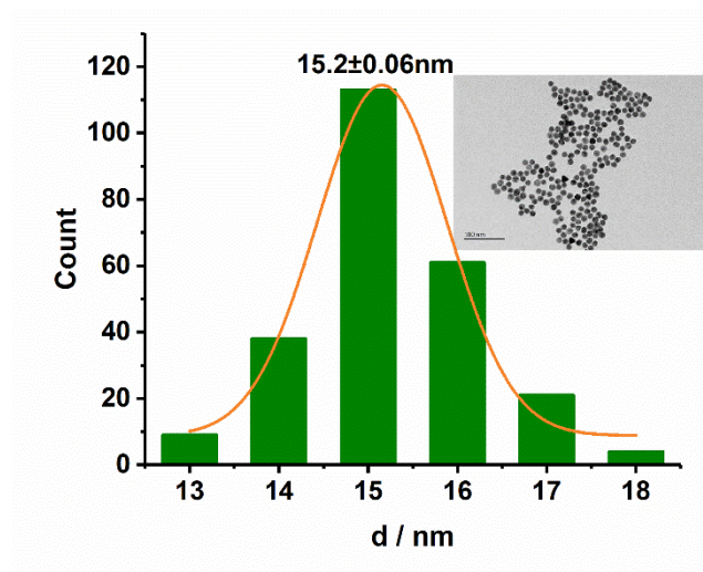
Figure S1. Size distribution of AuNPs with average diameter of 15.2 \pm 0.06 nm.
