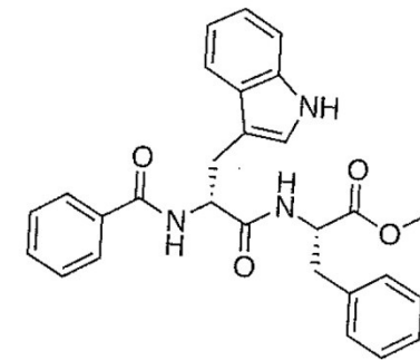
(2S,2'R)-6
