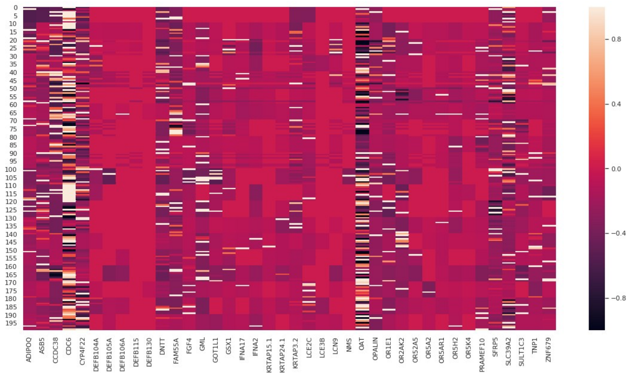
Supplementary Figure 2. Heatmap of a subset of samples of each primary site for the top 40 genes.
