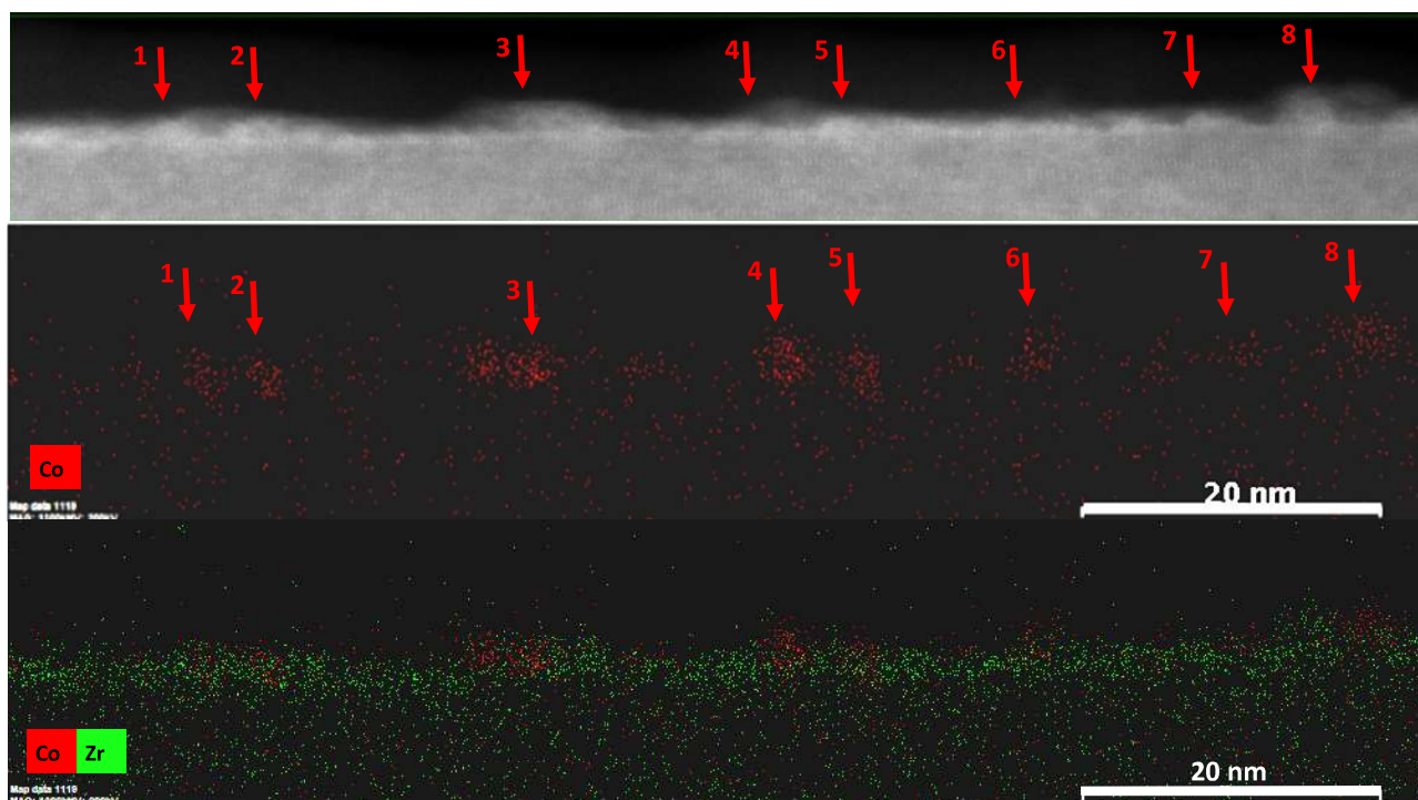
Figure S1. STEM with an EDS mapping verifying the Co islands with BZO region on the 4 nm thick sample with the numbers in the STEM referring to their respective regions in the EDS mapping
