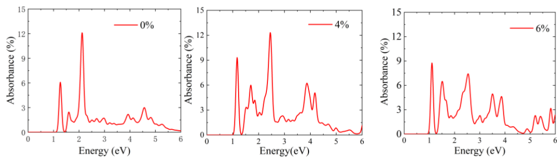
Fig. S1 Absorbance spectrum of Ti 2 CO 2 under tensile strains of 0%, 4% and 6%.
