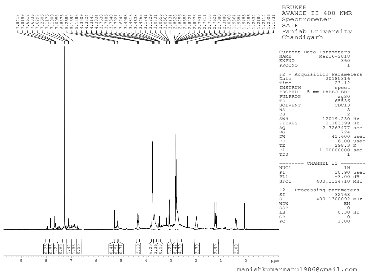
Fig. S2: 1 H NMR spectrum of 6
