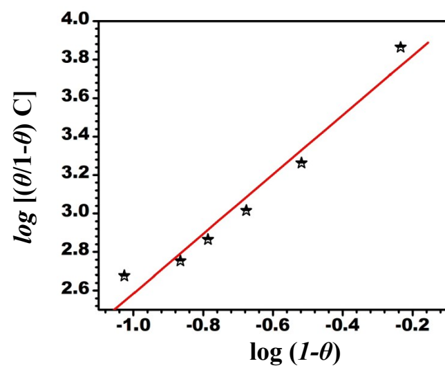
Figure S5. Flory-Huggins isotherm
