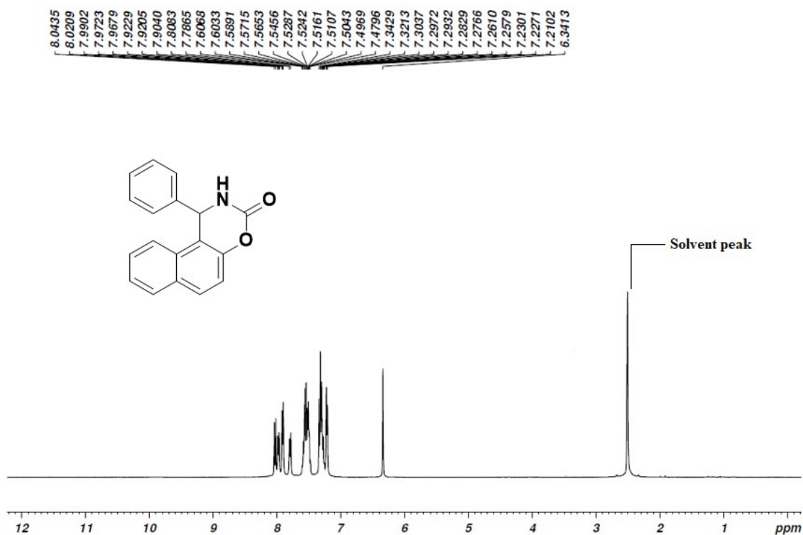
Figure S1. 1 H NMR Spectrum of compound
