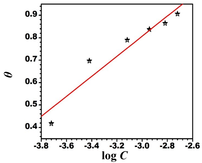
Figure S3. Temkin isotherm
