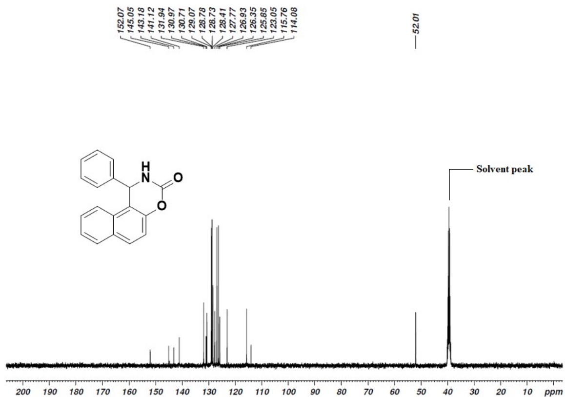
Figure S2. ^{13}\text{C} NMR Spectrum of compound
