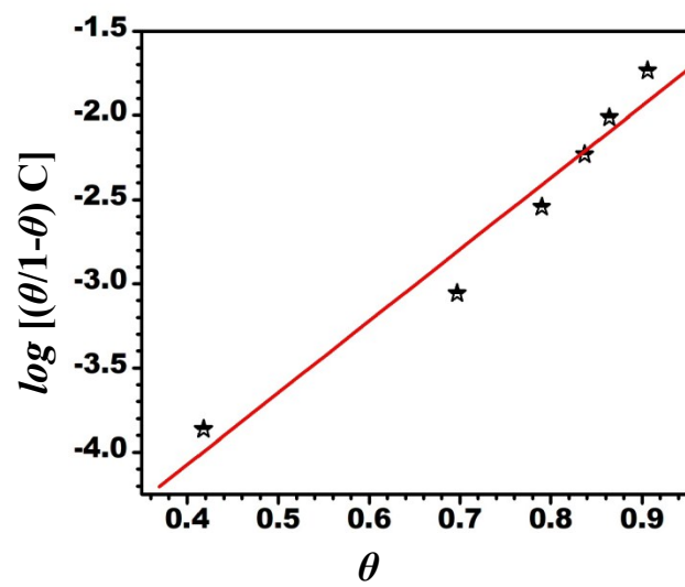
Figure S4. Frumkin isotherm
