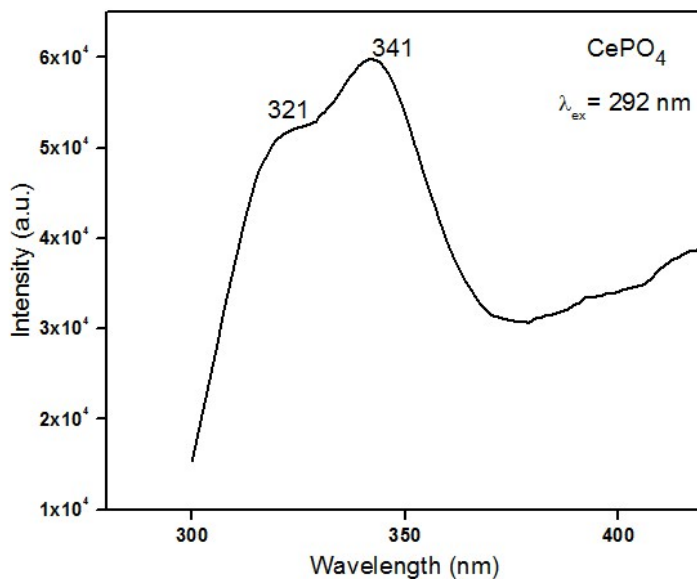
Figure S1: Photoluminescence emission spectra of pure CePO 4 , λ ex = 292 nm
