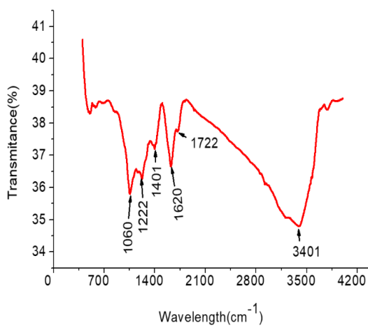
Fig S1. FTIR of GO
