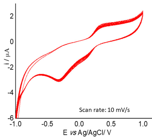
Fig. S3. Stability of PANI/ZnO-starch-rGO immobilized in nafion film modified GCE
