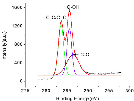
Fig S2. XPS of GO
