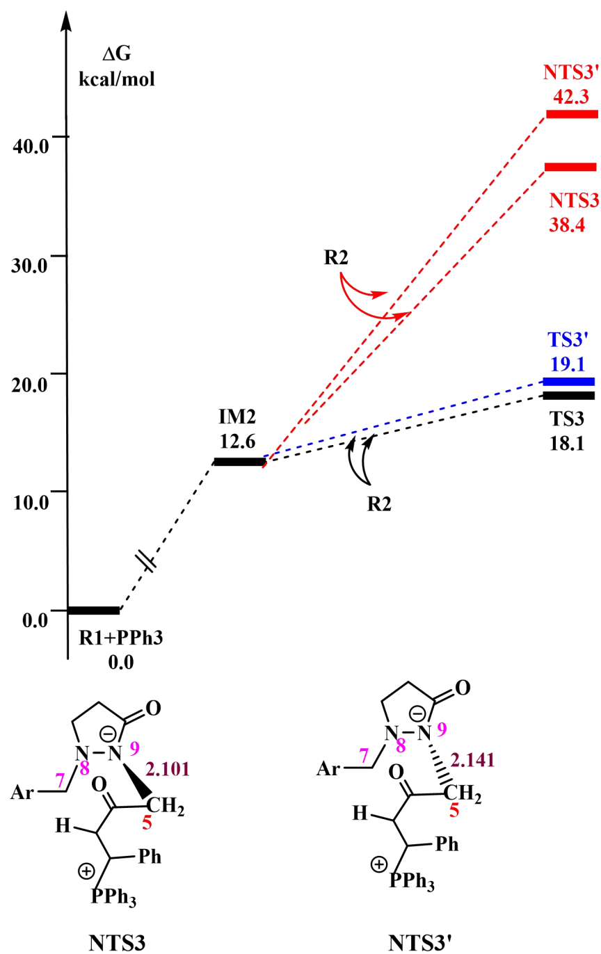
Fig. S2 Free energy profile and optimized structures for the addition of R2 to IM2 (the addition of the N9 atom to the C5 atom). The solvation-corrected relative free energies are given in kcal/mol. The bond lengths are given in Å.
