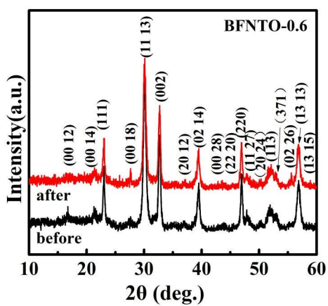
Figure S2 XRD patterns of BFNTO-0.6 sample before and after the photocatalytic RhB degradation.
