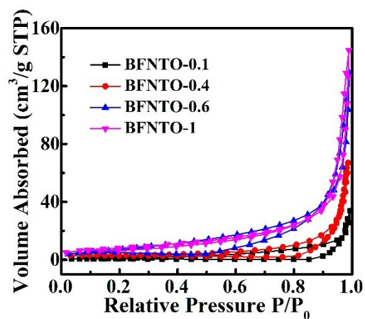
Figure S1 Adsorption-desorption isotherms of BFNTO samples.
