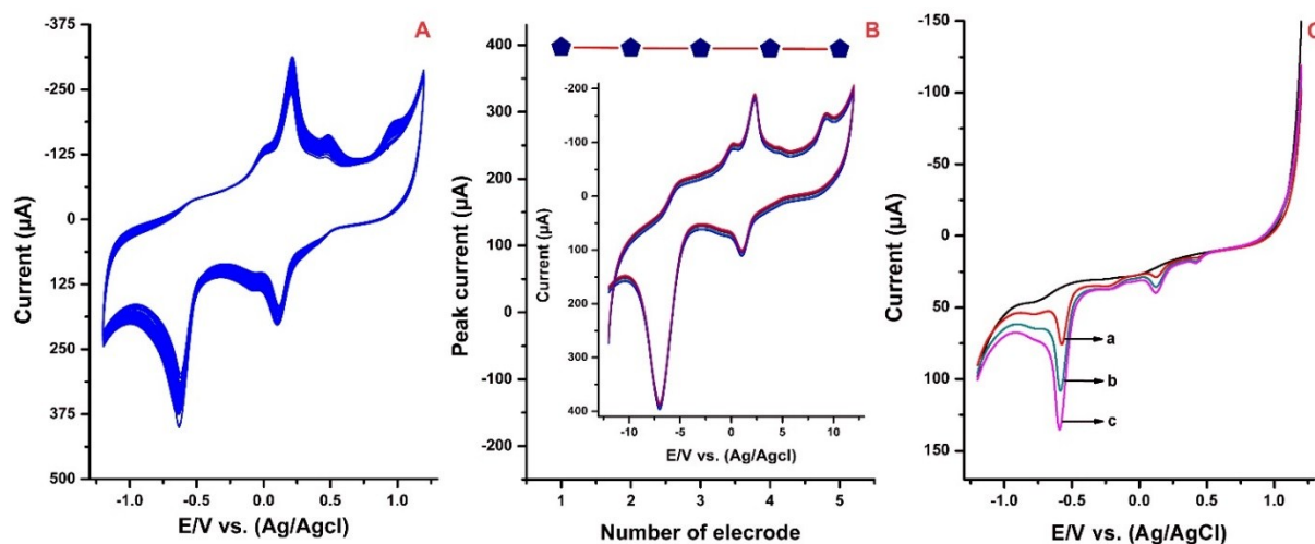
Fig S1. (A) Cyclic stability test (B) Reproducibility studies with linear plot (Inset) and (C) Real sample analysis (a) 9 \mu\text{M} (b) 15 \mu\text{M} , and (c) 22 \mu\text{M} .
