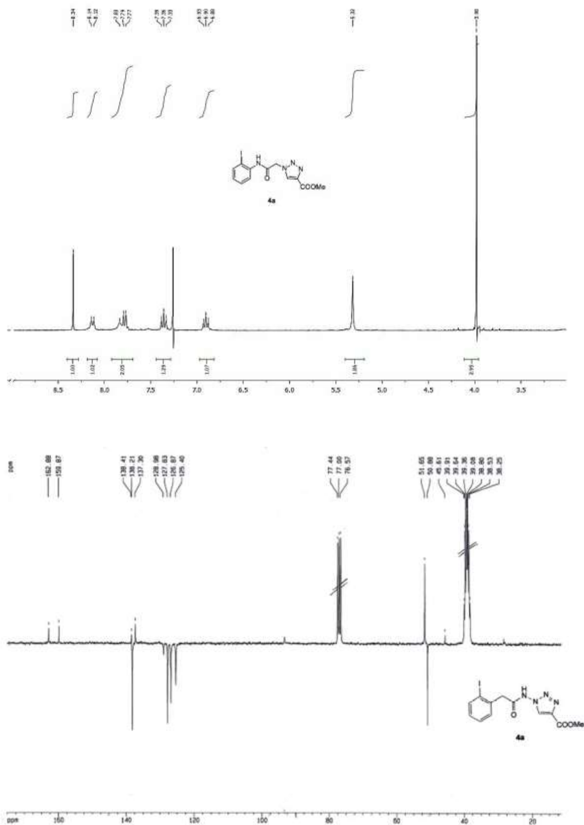
^1\text{H} - and ^{13}\text{C} -NMR spectra of compounds 4a , 5a , 4b , 5b , 4c , 5c , and 6 Figure S3. ^1\text{H} - and ^{13}\text{C} -NMR spectra of compounds 4a , 5a , 4b , 5b , 4c , 5c , and 6 .
