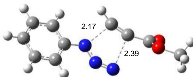
Figure S6. Geometrical parameters and structure of the regioisomeric transition states of the 1c + 2 reaction leading the 4 and 5 cycloadducts (OPBE /LANLDZ)
