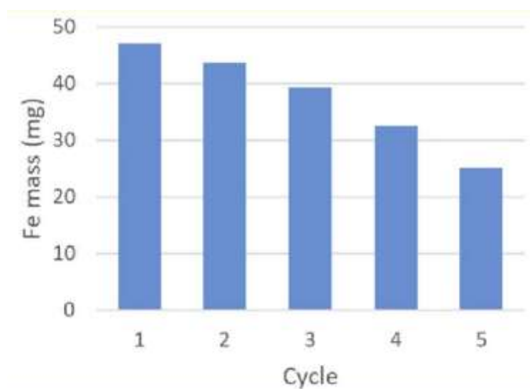
Figure S3. Amount of Fe 3 O 4 NPs recovered after each cycle of the cycloaddition of 1c to 2 .
