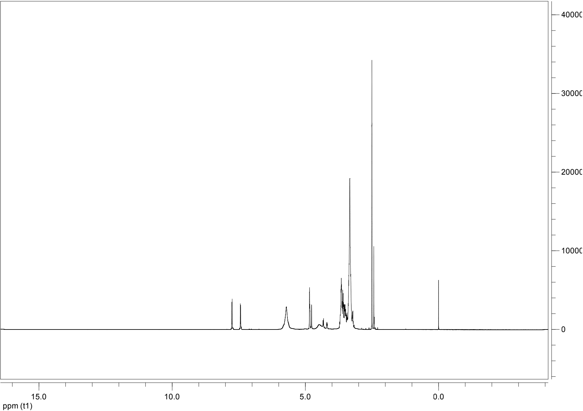
1 H NMR (600 MHz, DMSO-d 6 ) result of 6-OTS-β-CD
