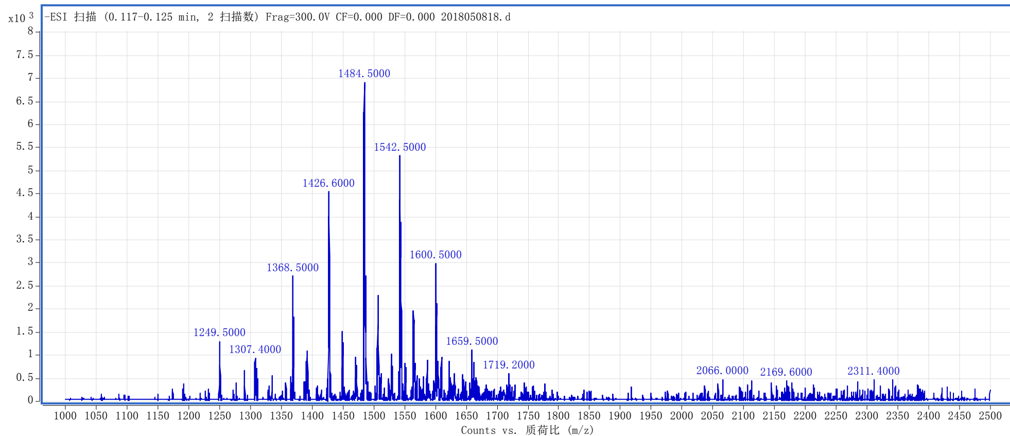
Mass spectrum of CMCDPN
