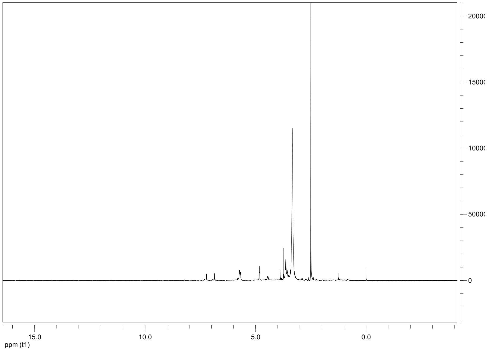
^1\text{H} NMR (600 MHz, \text{DMSO-d}_6 ) result of CDPN
