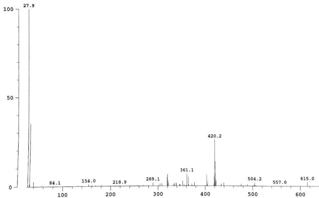
Figure S5: Mass spectrum for material 4
