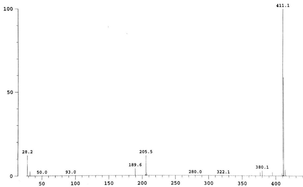
Figure S7: Mass spectrum for material 6
