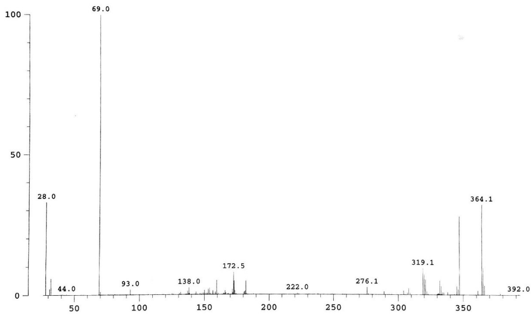
Figure S3: Mass spectrum for material 2
