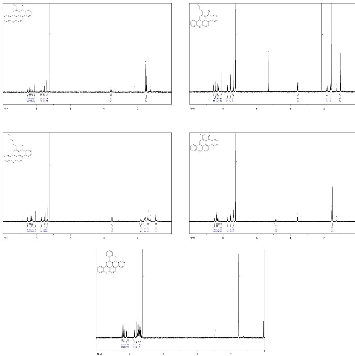
Figure S2: ^1\text{H} NMR spectra for the novel compounds synthesized in this study prior to sublimation.
