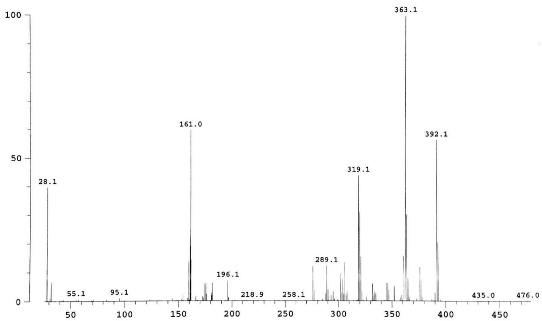
Figure S4: Mass spectrum for material 3
