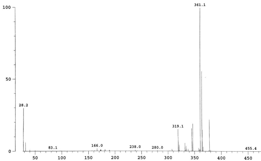
Figure S6: Mass spectrum for material 5
