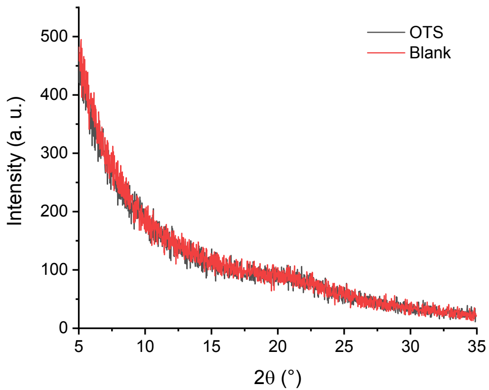
Figure S1: X-ray diffraction (XRD) scans of thin films of 6 on octyltrichlorosilane (OTS) modified SiO 2 and a blank control with no film.
