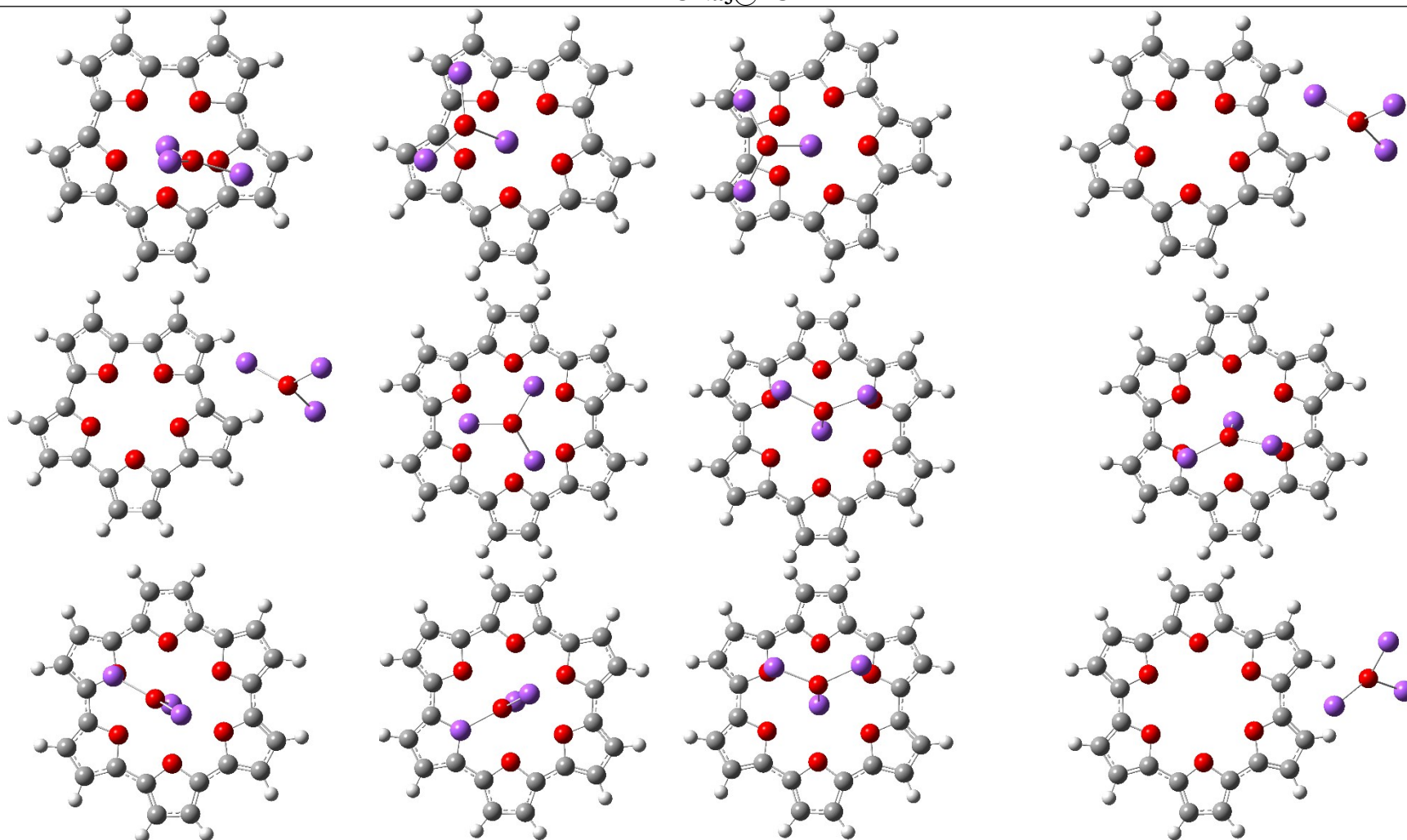
Fig. S1b. All the possible optimized geometries of \text{ONa}_3@\text{nCF} complexes.
