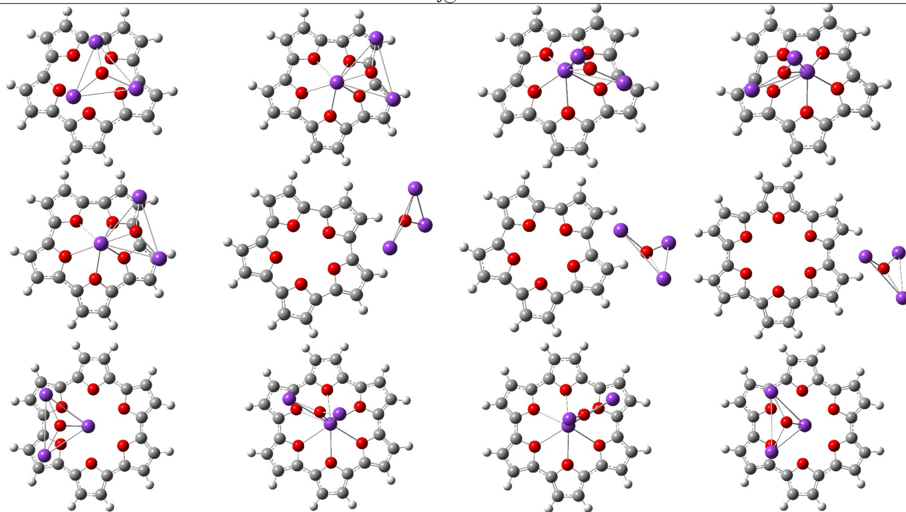
Fig. S1c. All the possible optimized geometries of \text{OK}_3@n\text{CF} complexes.
