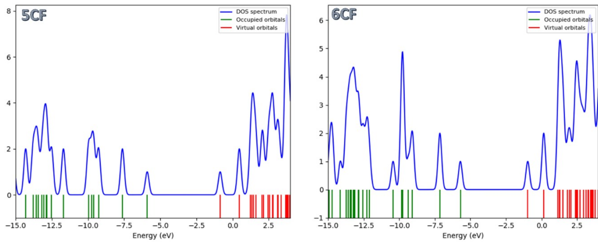
Figure S3. DOS spectra of isolated nCF.
