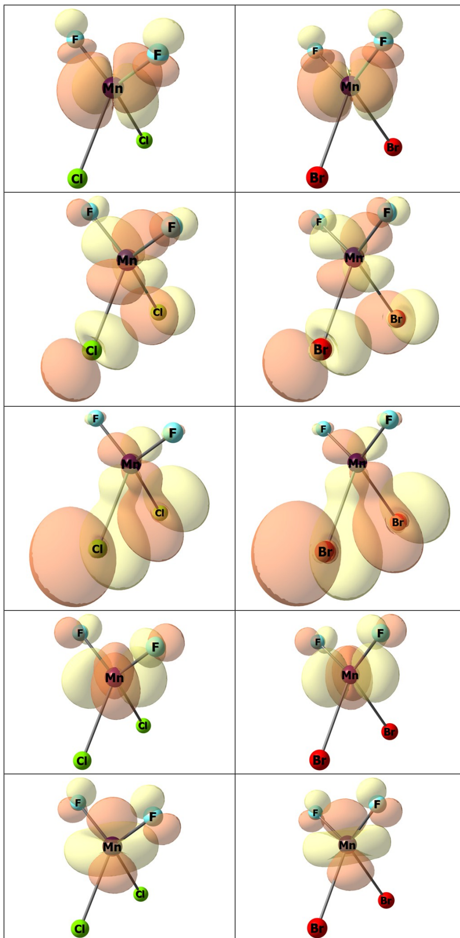
Fig. S4. Molecular orbitals of [\text{MnX}_2\text{F}_2] (X = Cl, Br) involved in the CASSCF calculations. Surface isovalue = 0.03 a.u.
