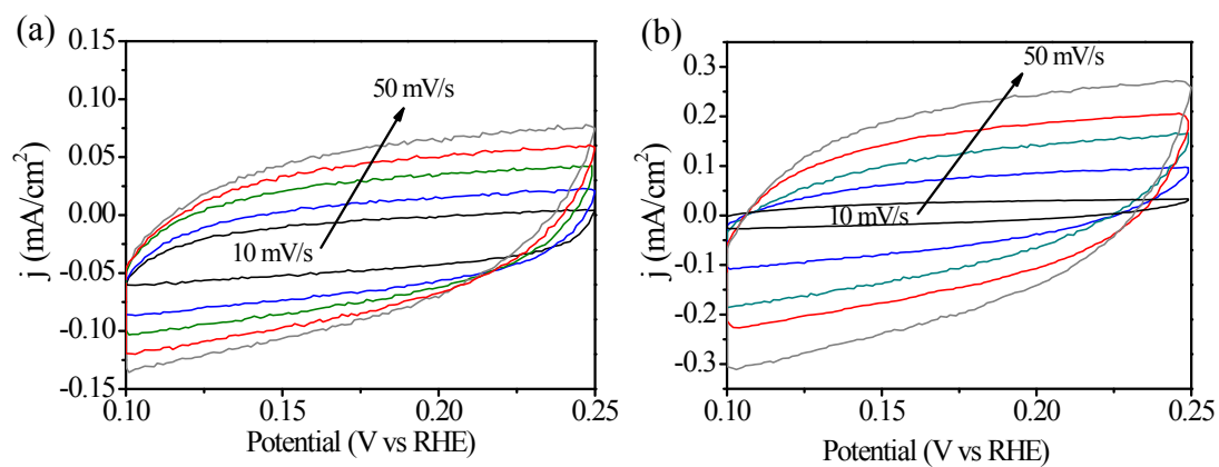
Fig. S1 (a), (b) CV curves of MoS 2 and P-MoS 2 -2 nanosheets in the region of 0.10-0.25 V vs. RHE.
