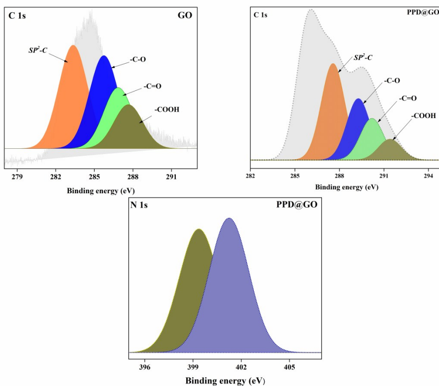
Figure S1 XPS spectra of C 1s of GO and PPD@GO, N 1s spectra of PPD@GO.
