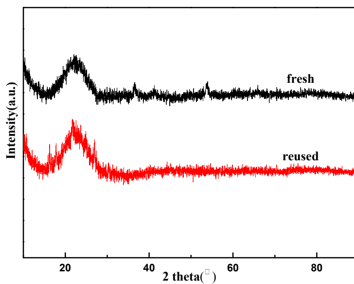
Fig. S2 XRD patterns of fresh and reused MoO 2 /ZrO 2 -SiO 2 catalysts.
