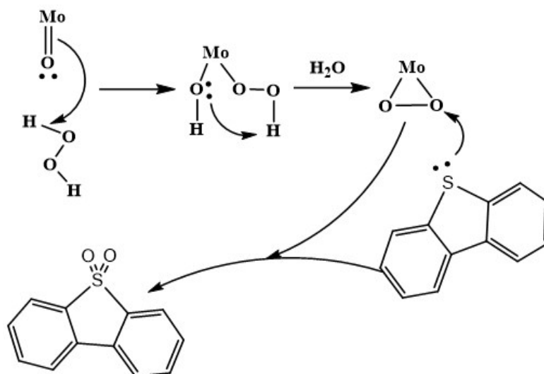
Fig. S1 The reaction mechanism of sulfur containing compounds.
