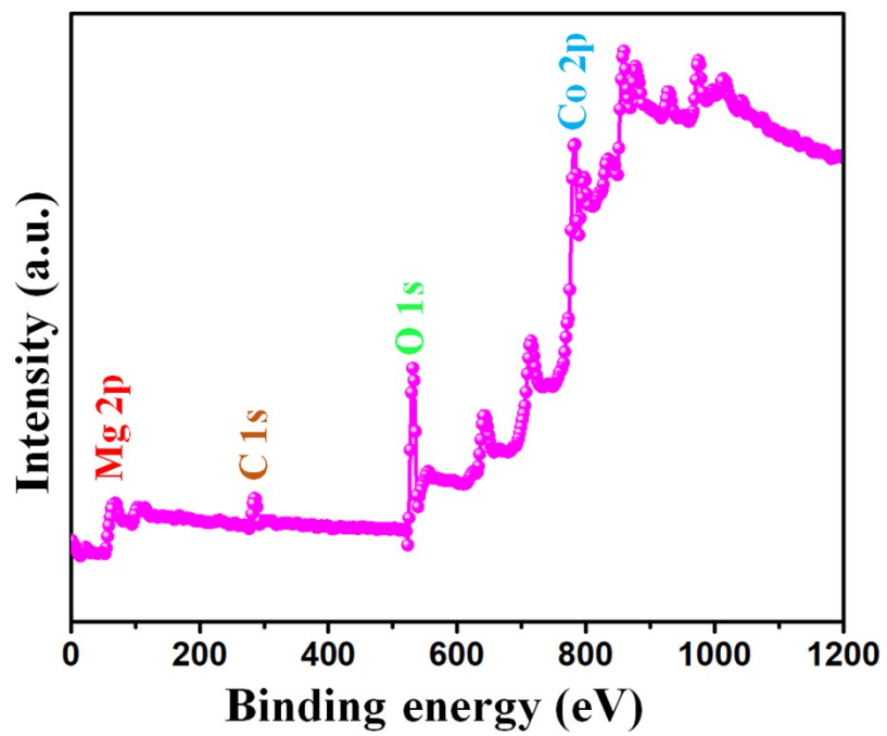
Fig. S1 XPS survey spectrum of MCO NFAs
