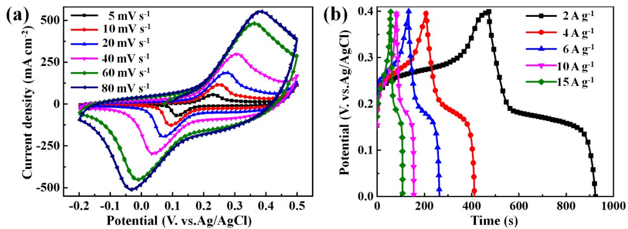
Fig. S2 (a,b) CV and GCD curves of MCO NFAs electrode on nickel foam in 2 M KOH electrolyte solution.
