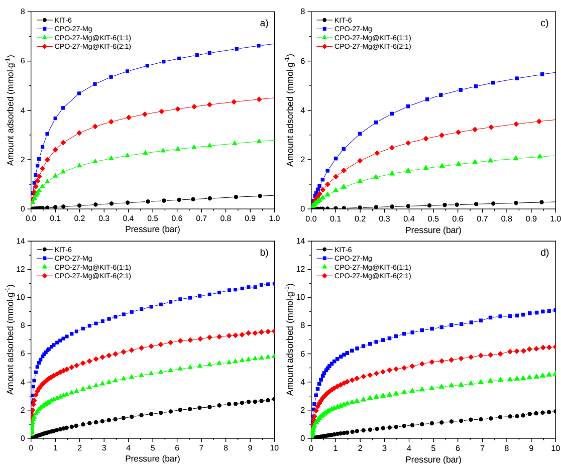
Figure S1. CO 2 adsorption isotherms until 10 bar of KIT-6, CPO-27-Mg, and CPO-27-Mg@KIT-6(1:1) and (2:1) at (a-b) 323 K and (c-d) 348 K.
