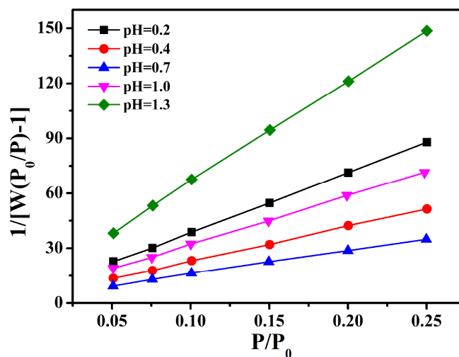
Fig.S1 Relationship curves between [W(P_0/P)-1]^{-1} and (P/P_0) for the WO 3 samples.
