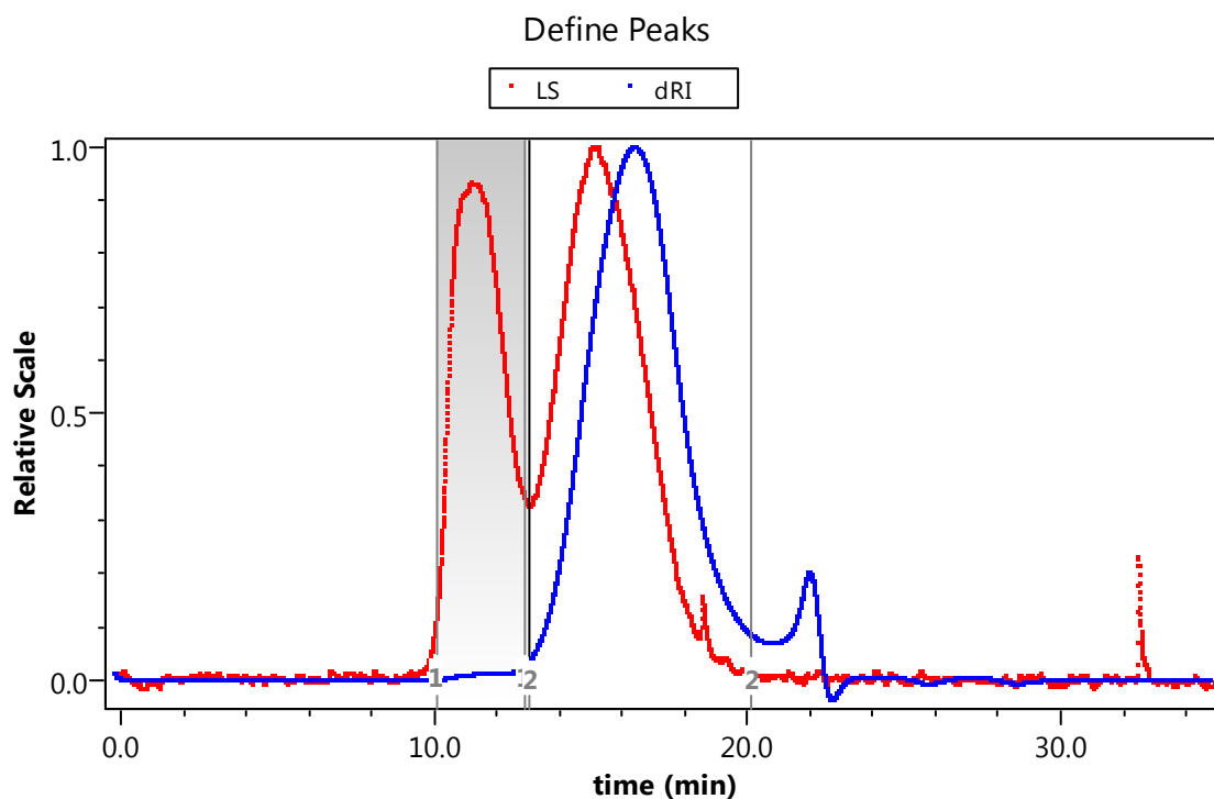
Fig. S1. GPC trace of PUE-A.
