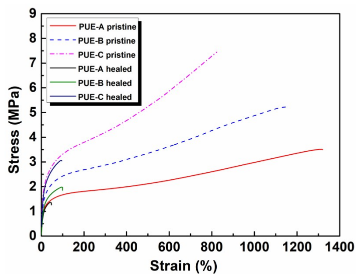
Fig. S5. Stress-strain curves of original and self-healed PUEs.
