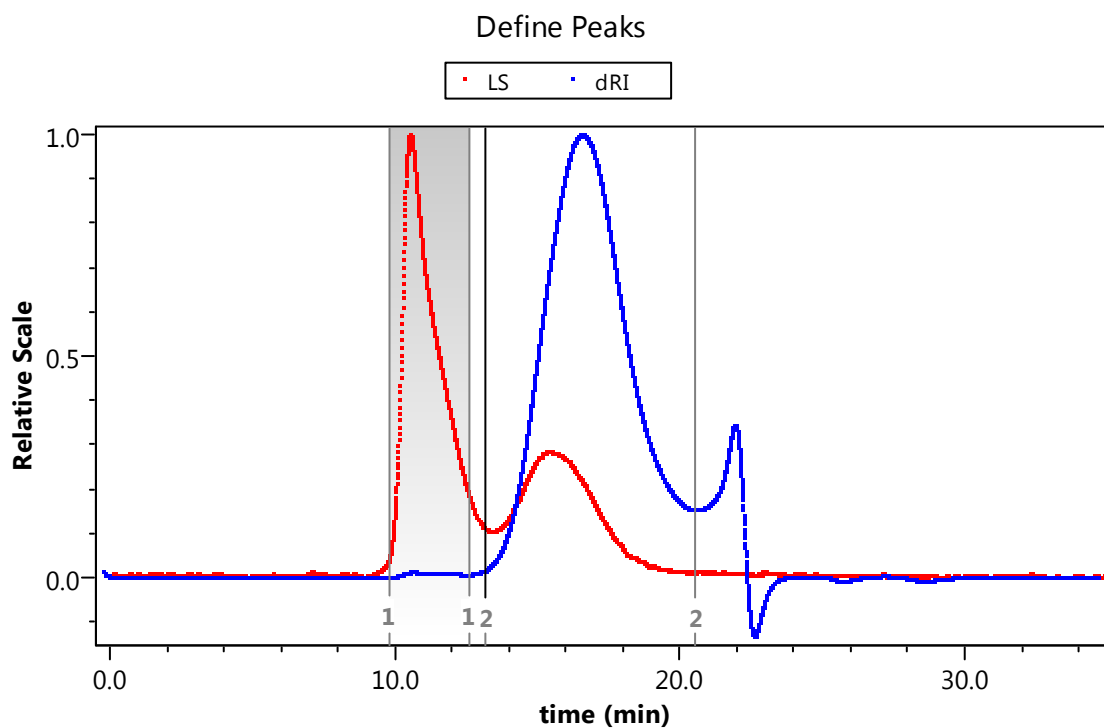
Fig. S2. GPC trace of PUE-B.
