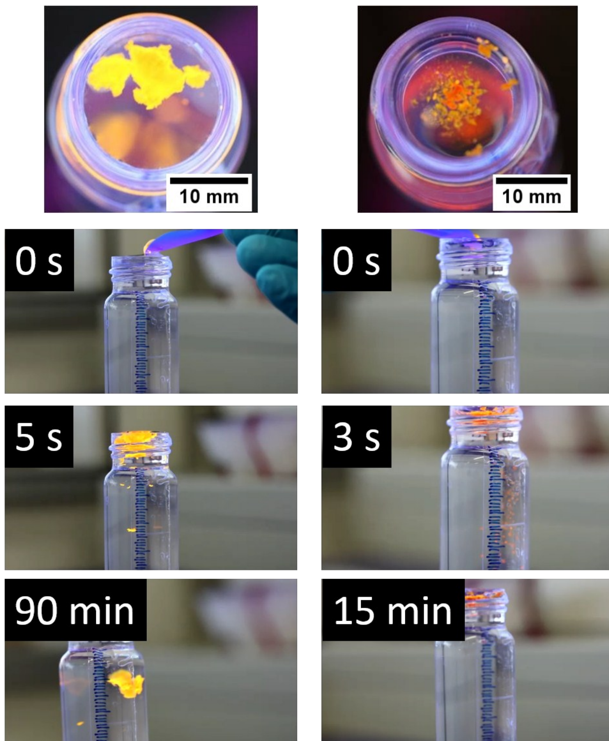
Figure S11. Rehydration experiment with silica modified (left) and unmodified (right) CdSe/CdS network structures shown at different time points (measured from addition of aerogel to water) under UV illumination as top and side view.
