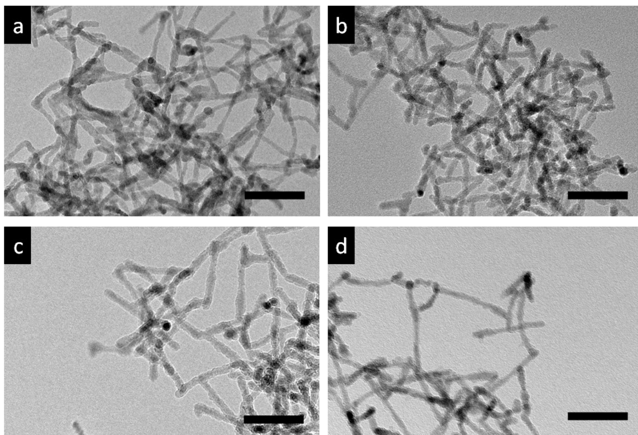
Figure S3. TEM micrographs of silica modified CdSe/CdS nanorod networks with increasing amount of ammonia added for hydrolysis of TEOS, (a) no \text{NH}_3 added, (b) 1 \mu\text{L} , (c) 5 \mu\text{L} , (d) 20 \mu\text{L} , scale bars correspond to 50 nm.
