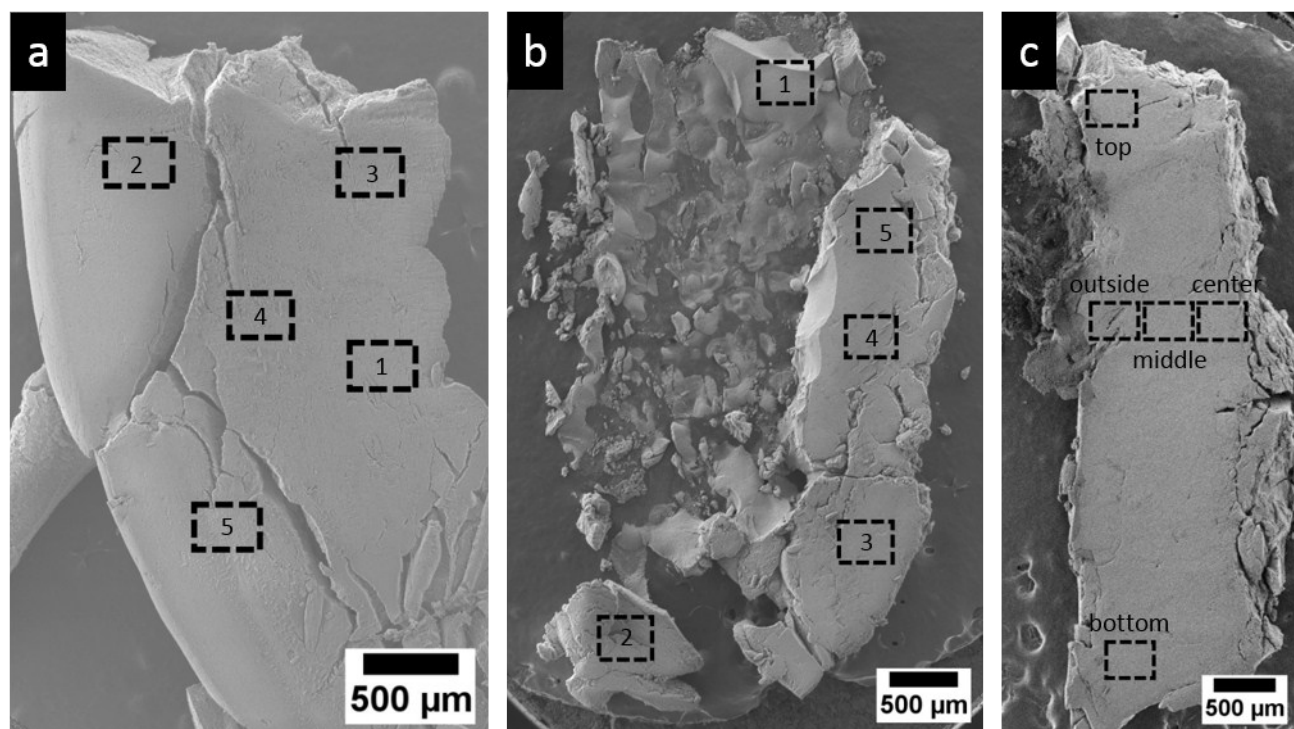
Figure S4. Overview SEM micrographs of samples with measurement positions for elemental distribution by EDX for different ratios of Si/Cd, (a) no TEOS added, (b) 1/1, and (c) 2/1. Pictures are assembled from two single measurements each.
