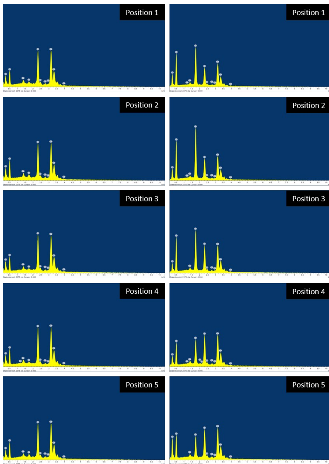
Figure S5. EDX spectra of unmodified (left) and modified (Cd/Si 1:1, right) networks at different measurement positions as indicated in figure S4.
