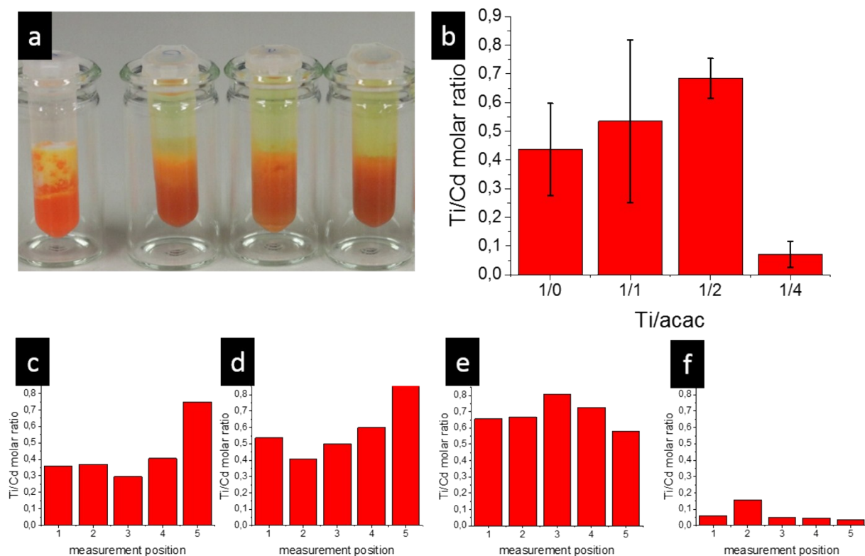
Figure S9. Influence of acetylacetone on homogeneity of titania shell. (a) Real color photographs of CdSe/CdS nanorod networks with titania shell employing different ratios of Ti/acac (from left to right 1/0 – 1/1 – 1/2 – 1/4), (b) Ti/Cd molar ratios by local EDX measurement in these networks with deviation derived from measurements at different positions of the network. Individual Ti/Cd molar ratios measured at different positions of the network for Ti/acac ratios (c) 1/0, (d) 1/1, (e) 1/2 and (f) 1/4.
