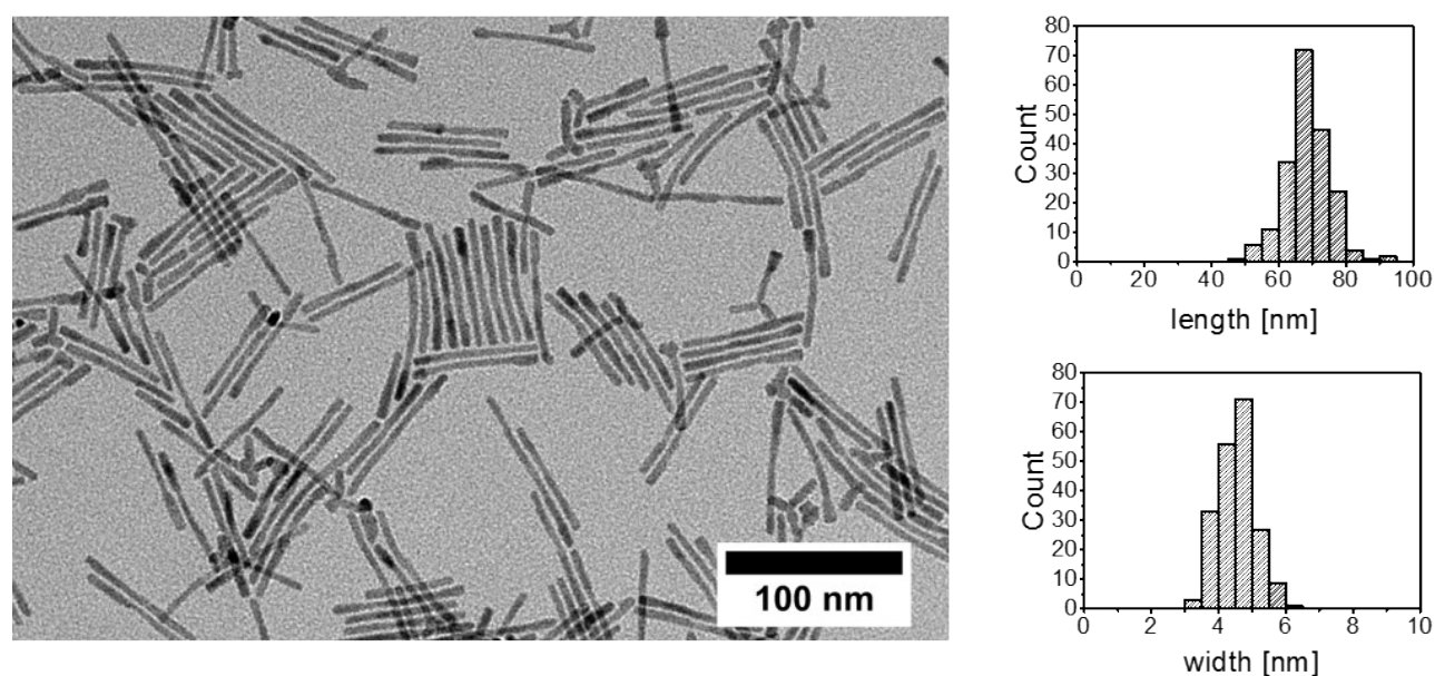
Figure S1. TEM micrograph and size distribution (measured for 200 particles) of CdSe/CdS nanorods used for production of networks.
