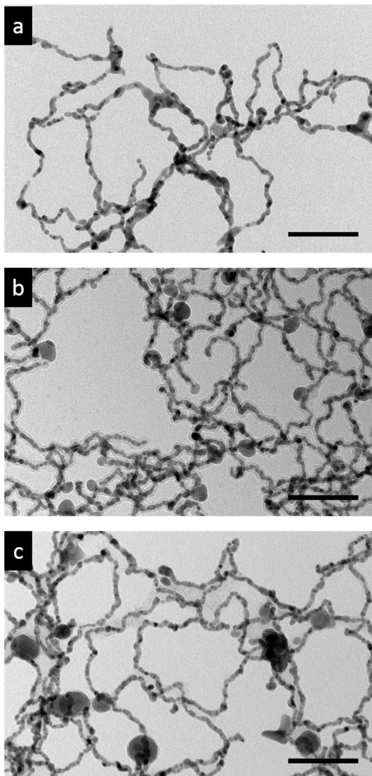
Figure S10. Au and Ag nanoparticle based network (a) before and (b) after silica shell growth with APTMS linker and (c) without APTMS linker added in the modification step. Scale bars correspond to 100 nm.
