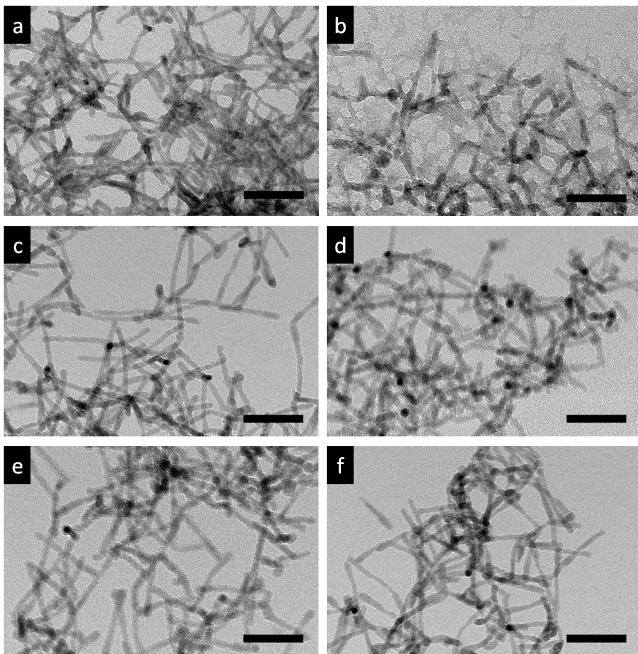
Figure S2. TEM micrographs of silica modified CdSe/CdS nanorod networks with increasing amount of water added for hydrolysis of TEOS, (a) neither water nor ammonia added, (b) no water added, (c) 45 \mu\text{L} , (d) 90 \mu\text{L} , (e) 360 \mu\text{L} , (f) 900 \mu\text{L} water added, scale bars correspond to 50 nm.
