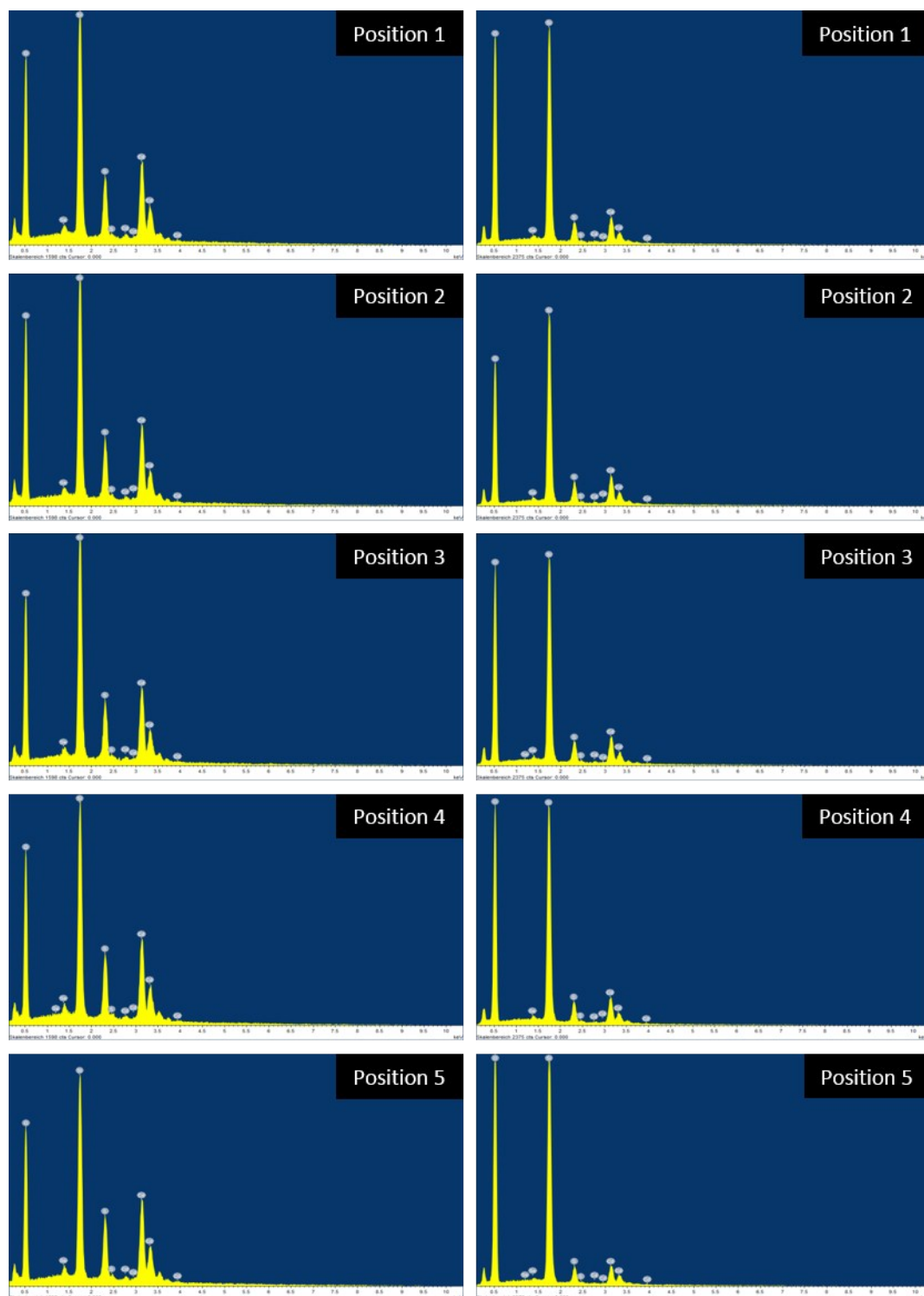
Figure S6. EDX spectra of modified networks, Cd/Si 1:2 (left) and Cd/Si 1:10 (right), at different measurement positions as indicated in figures 3 and S4.
