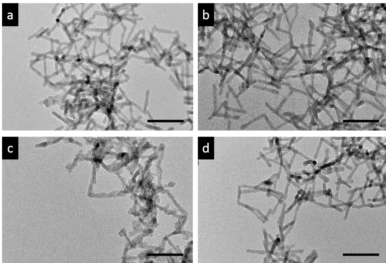
Figure S8. TEM micrographs of titania modified CdSe/CdS nanorod networks with increasing amount of acetylacetonate added to the modification. Ti/acac-ratio: (a) 1/0, (b) 1/1, (c) 1/2, (d) 1/3. Scale bars correspond to 50 nm.
