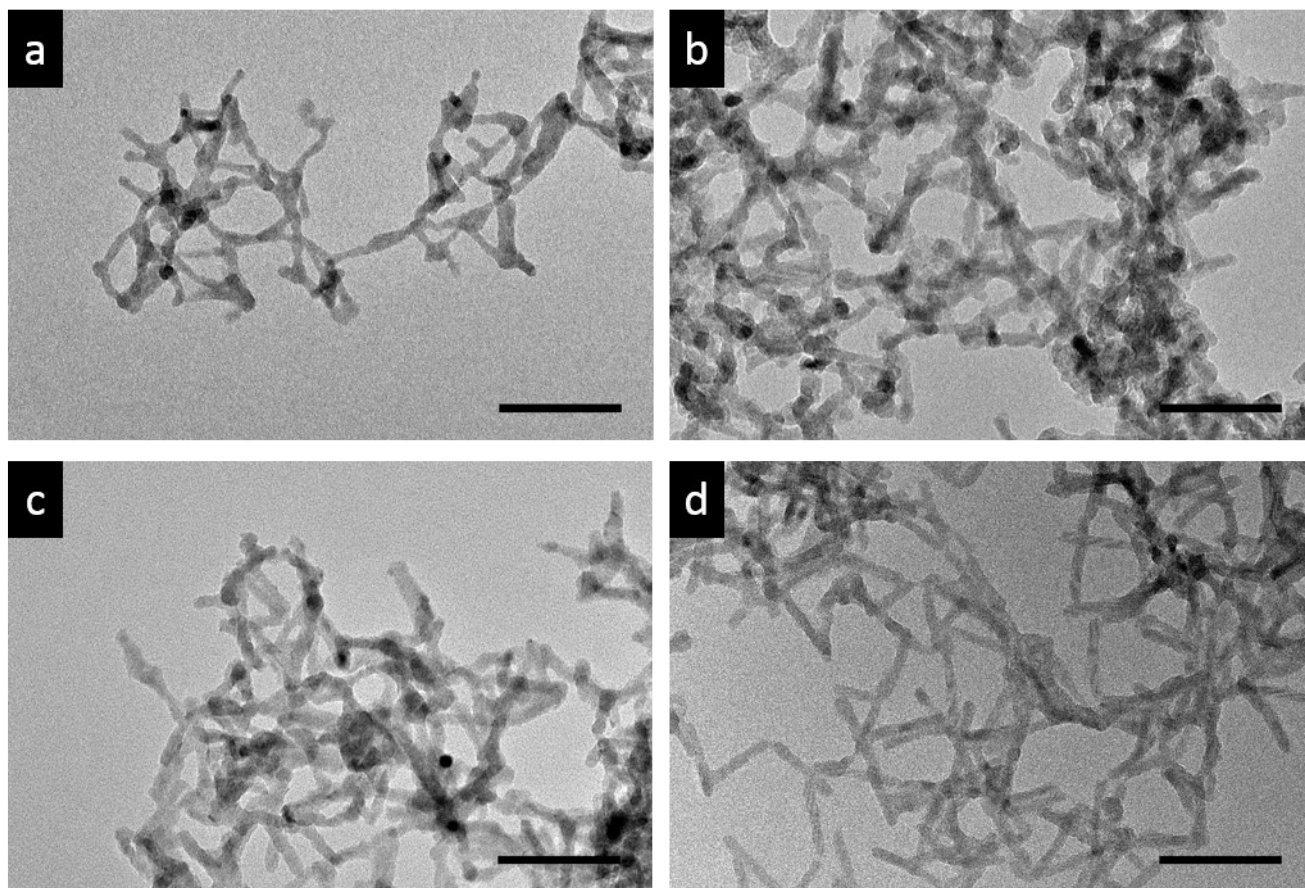
Figure S7. TEM micrographs of titania modified CdSe/CdS nanorod networks with increasing ratio of titania precursor added to cadmium content of the network, (a) 0/1, (b) 1/1, (c) 2/1, (d) 10/1. Scale bars correspond to 50 nm.
