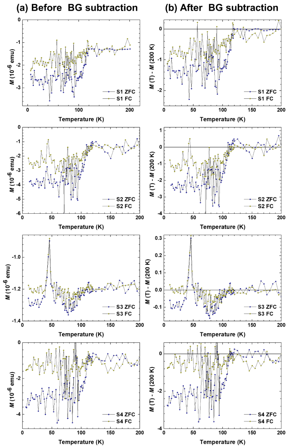
Figure S1. The diamagnetic Meissner signal of films S1, S2, S3 and S4 at H = 100 Oe. (a) Before back ground (BG) subtraction. (b) After BG subtraction.
