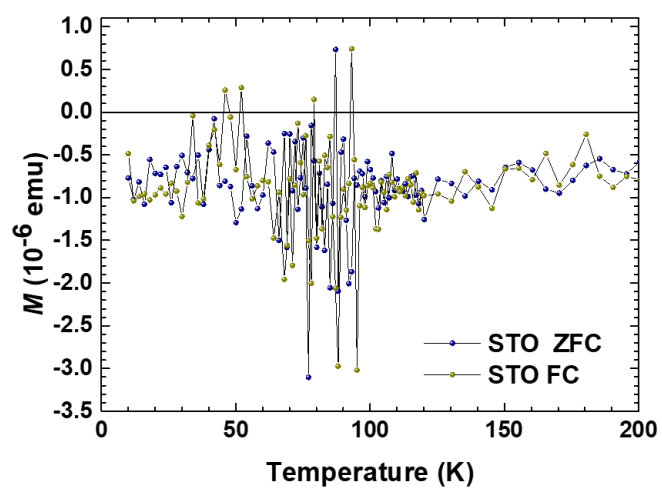
Figure S2 Temperature dependence of magnetization for an STO substrate at H = 100 Oe.
