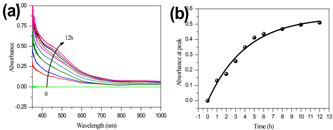
Fig. S2. (a) UV-vis absorption spectra of m -TiO 2 /N-CQDs photoanodes at immersion time range of 0-12 h. (b) Plots of absorbance at 450 nm as a function of immersion time.
