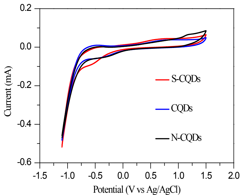
Fig. S1. CV curves of different CQDs on a platinum electrode in 0.1 M tetrabutylammonium hexafluorophosphate in acetonitrile at a scanning rate of 50 mV s -1 .
