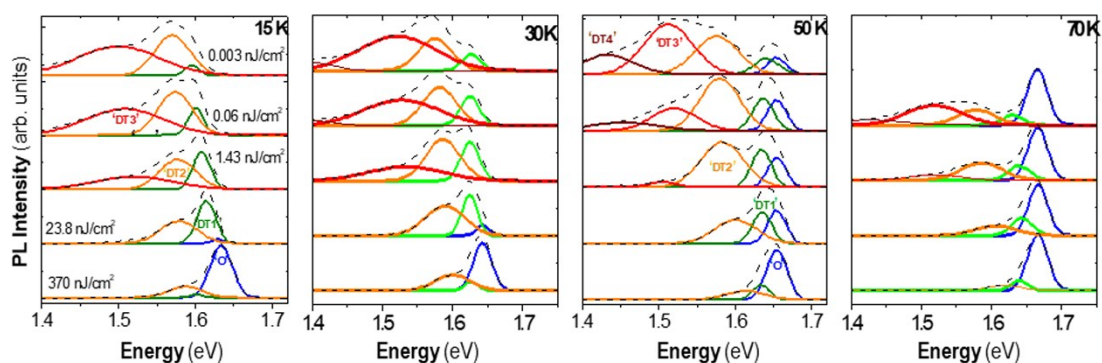
Figure S1 – Deconvolution of PL spectra as a function of Energy
