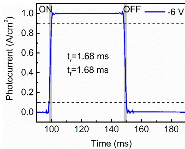
Figure S1. Transient photocurrent response ( J - t curve) of the resulting OPDs without MoO 3 at a pulse frequency of 10 Hz and -6 V bias.
