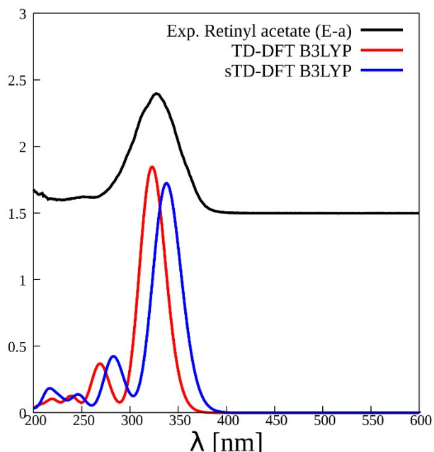
Figure S6. Comparison of computed UV-Vis spectra of retinyl acetate E-a using two methods: TD-DFT (red) and sTD-TDF (blue). Experimental spectrum is given in black for reference. Calculated spectra were shifted uniformly by -30 nm to match experimental spectrum visually.
