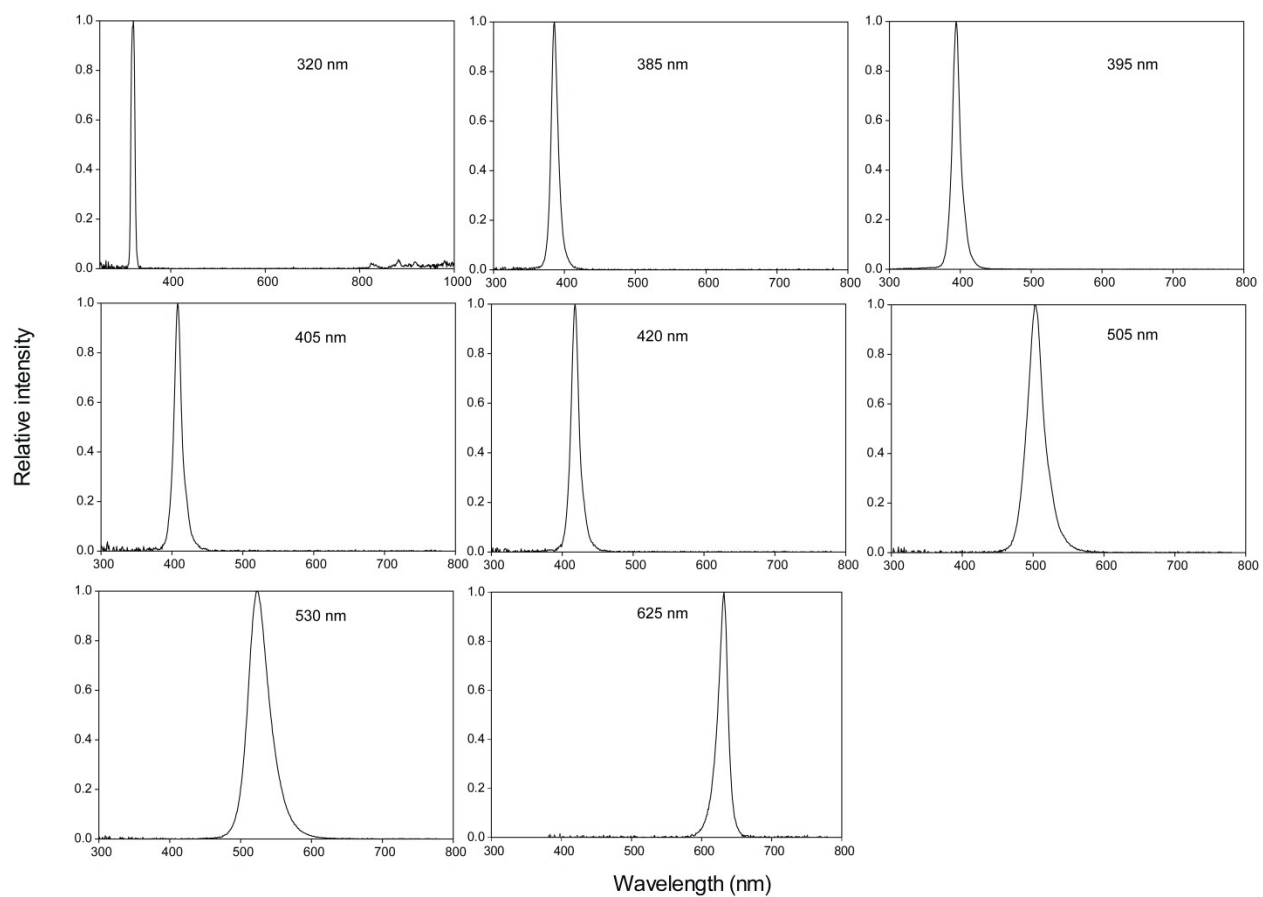
Figure S1. Emission spectrum of the screened UV wavelength (320, 385, 395, 405, 420, 505, 530 and 625 nm)
