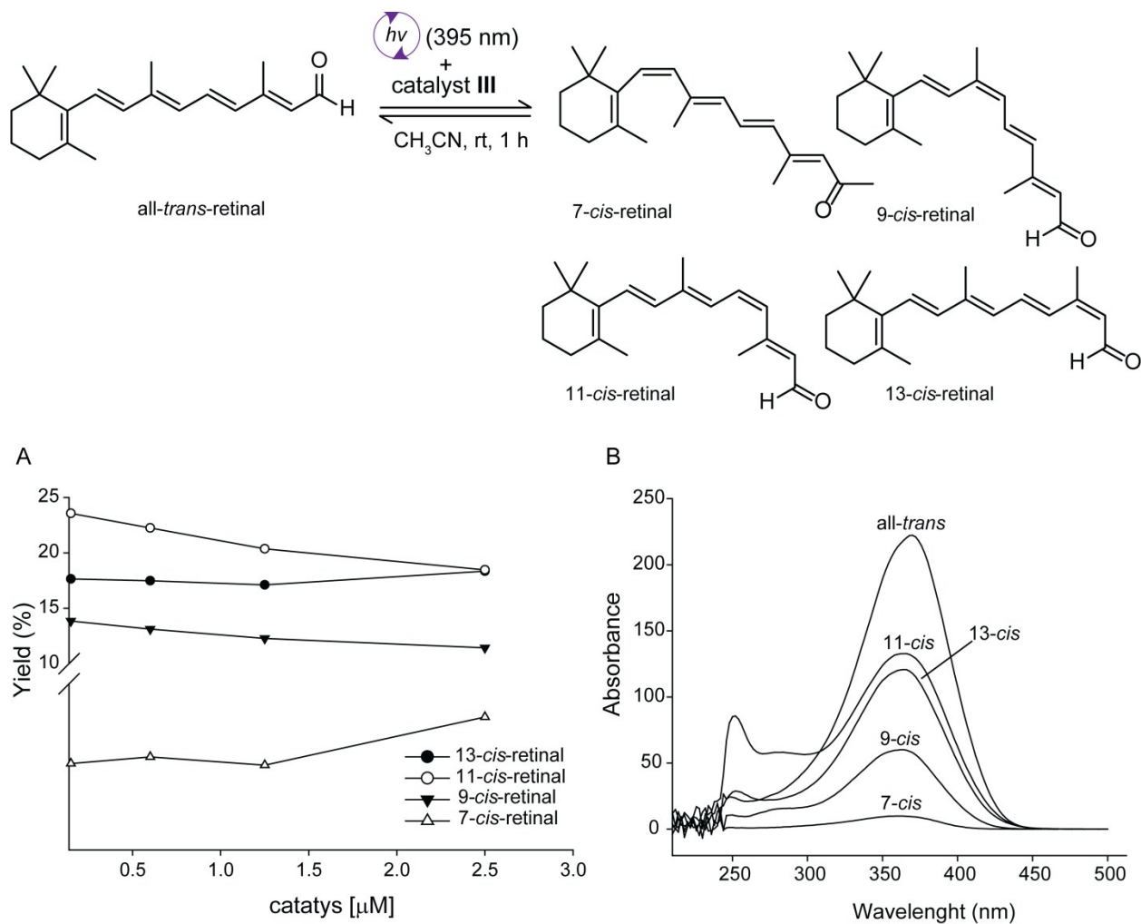
Figure S4. A) Catalyst III effect on the distribution of cis -retinal isomers. B) Absorbance spectra of all isomers.
