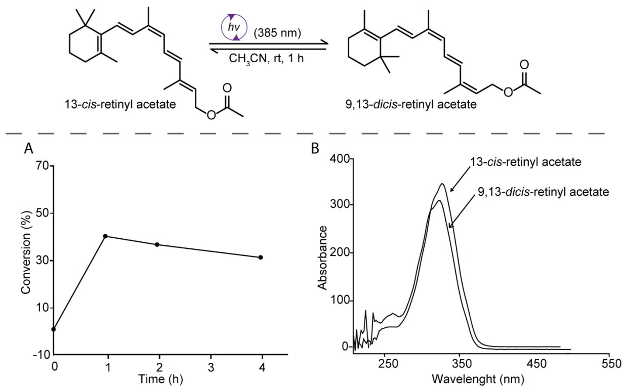
Figure S3. The relationship between the distribution of cis -retinyl acetate isomers. A) Time course of the reaction from 13- cis to 9,13- dicis . B) Absorbance spectra of 13- cis and 9,13- dicis isomers.
