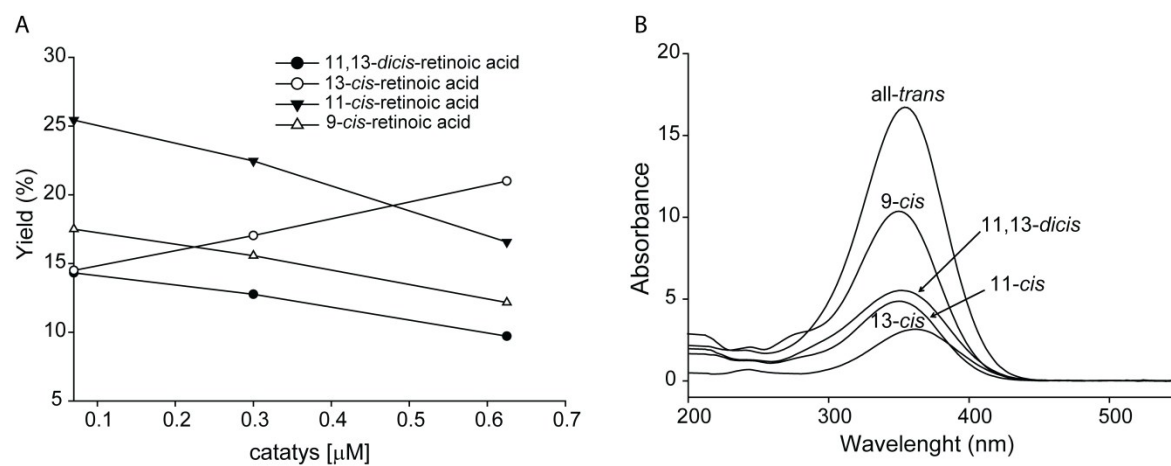
Figure S5. A) Catalyst III effect on the distribution of cis -retinoic acid isomers. B) Absorbance spectra of all isomers.
