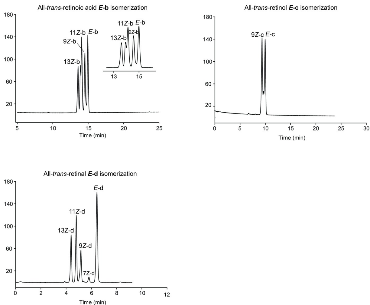
Figure S2. Representative HPLC chromatograms of a mixture of all- trans -retinoic acid E-b , all- trans -retinol E-c and all- trans -retinal E-d , obtained following irradiation treatment. 9Z-b , 9Z-c and 9Z-d represent the 9- cis isomer, 7Z-d represents the 7- cis isomer, 13Z-b and 13Z-d represent the 13- cis isomer, and 11Z-b and 11Z-d represent the 11- cis isomer.
