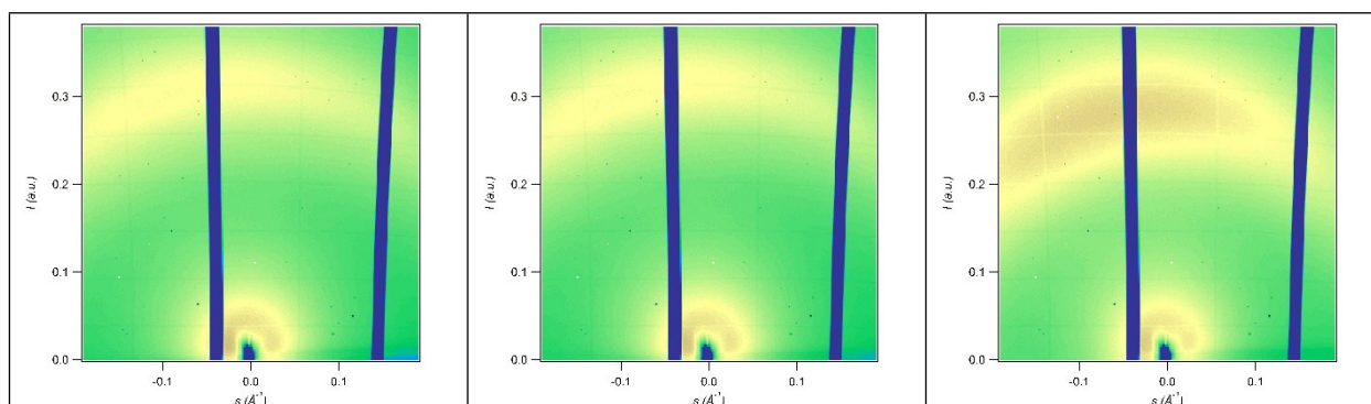
Fig. S1 Diffractograms of aqueous dispersions of PVCL/AAEM/VIm/(C8AzoSO 3 H) 25% , PVCL/AAEM/VIm/(C8AzoSO 3 H) 50% and PVCL/AAEM/VIm/(C8AzoSO 3 H) 100% : from left to right, respectively.
