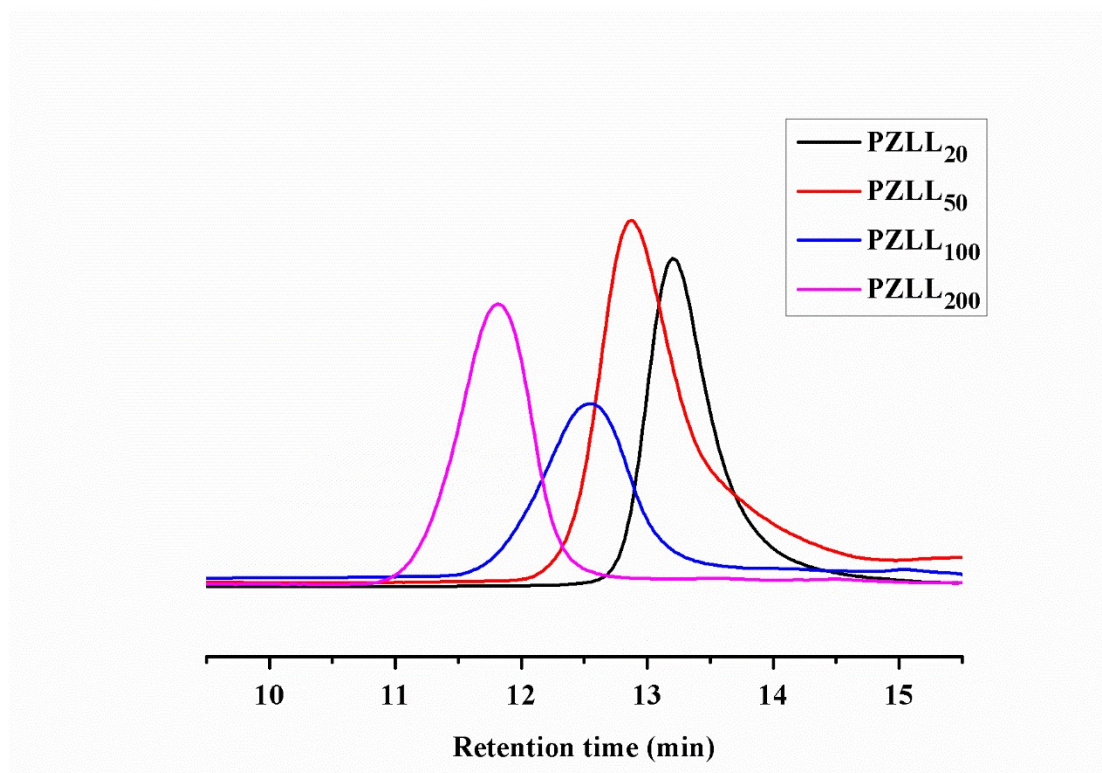
Fig. S3 GPC curves of PZLL 20 , PZLL 50 , PZLL 100 and PZLL 200
