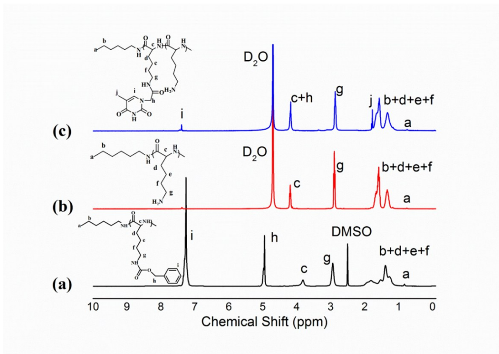
Fig. S2 ^1\text{H} NMR spectra of (a) PZLL, (b) PLL, (c) PLL-co-PTLL
