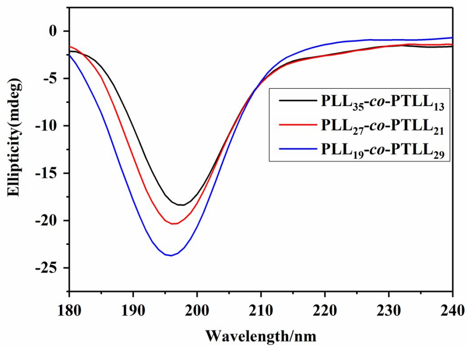
Fig. S4 CD spectrum of PLL 35 -co-PTLL 13 , PLL 27 -co-PTLL 21 and PLL 19 -co-PTLL 29
